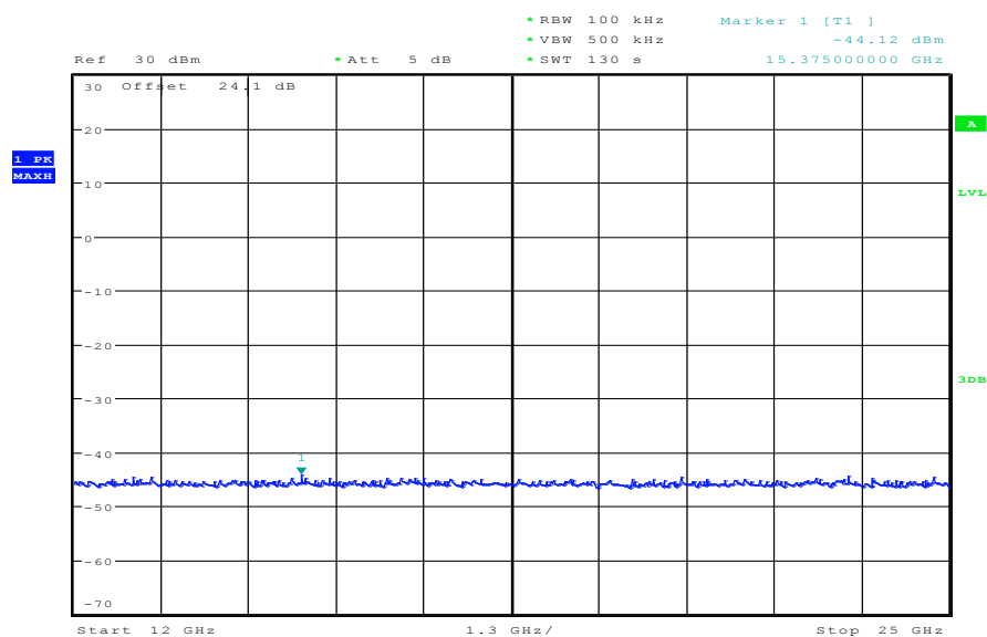
Plot 2: TX mode, lowest channel, 12 to 25 GHz
