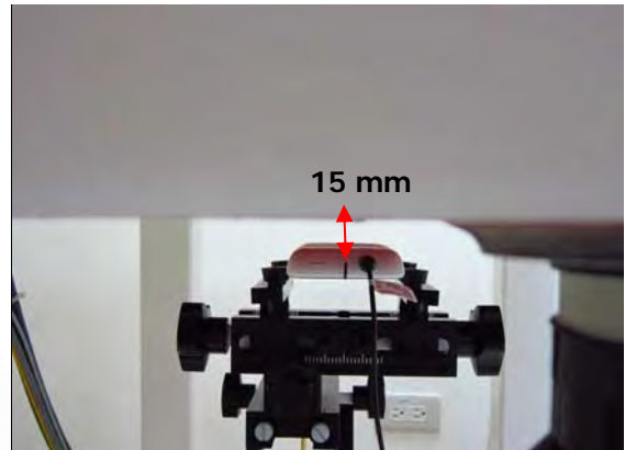
Fig.8 EUT Back side with Headset to flat phantom
