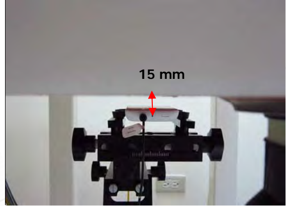
Fig.7 EUT Front side with Headset to flat phantom
