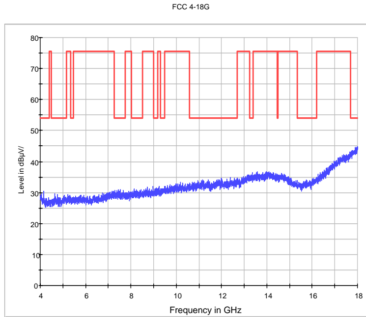
Fig.99. Radiated emission: 8DPSK, Channel 78, 4 GHz - 18 GHz
