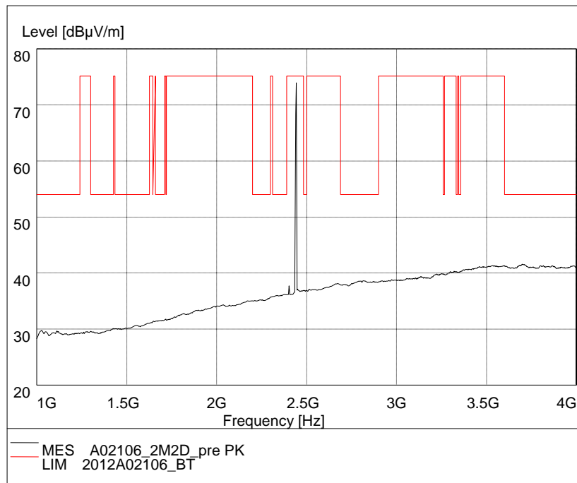
Fig.79. Radiated emission: \pi/4 DQPSK, Channel 39, 1 GHz - 4 GHz
