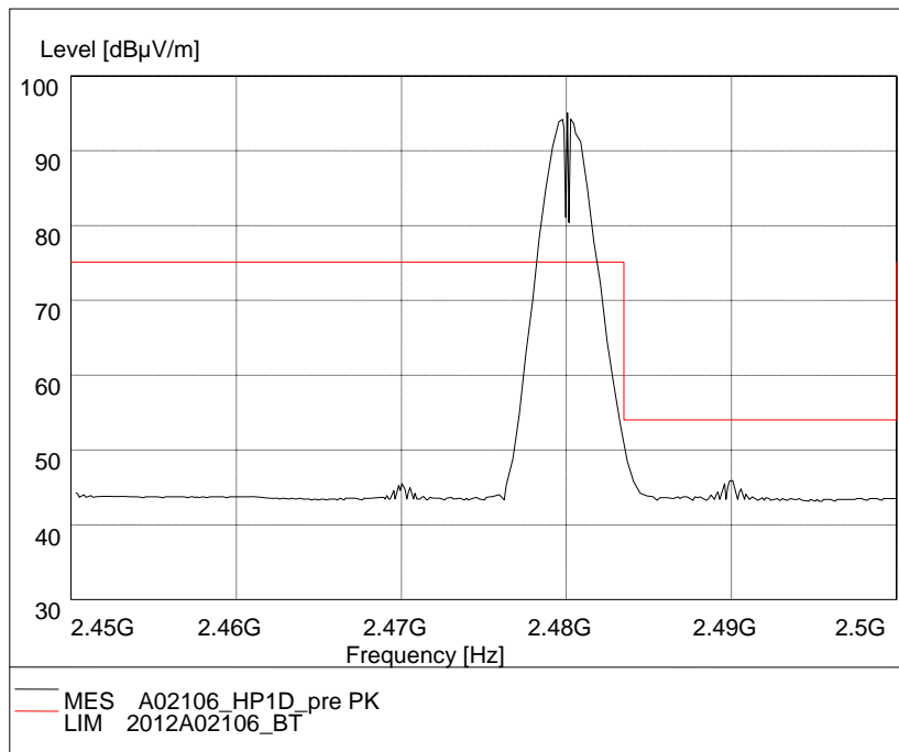
Fig.71. Radiated emission (Power) GFSK, high channel
