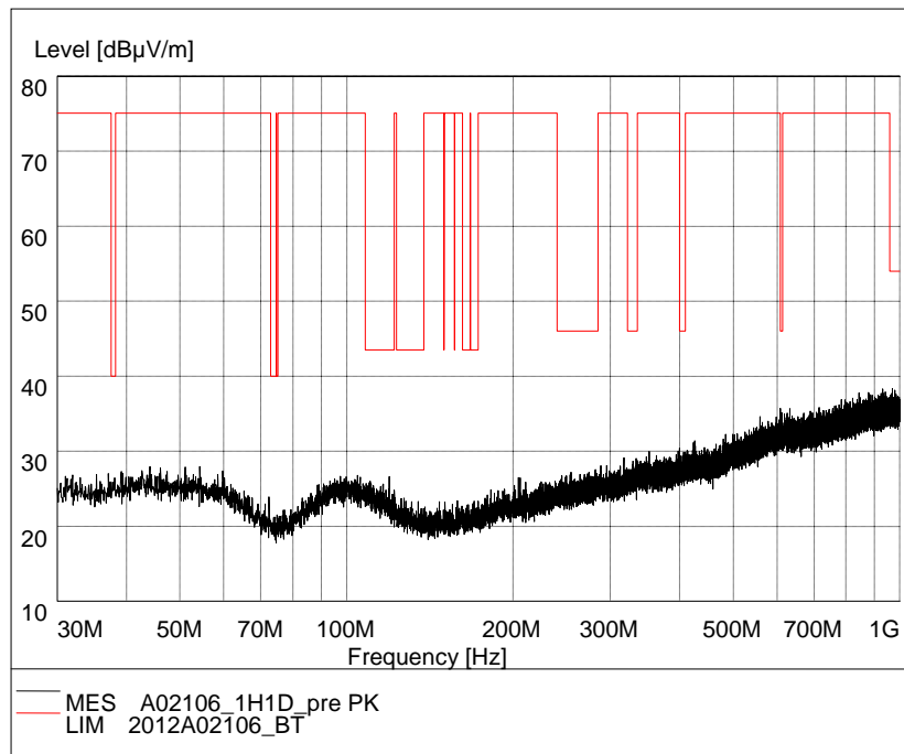
Fig.67. Radiated emission: GFSK, Channel 78, 30 MHz - 1 GHz
