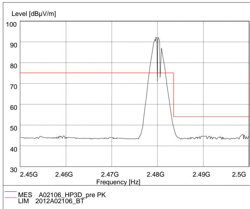
Fig.101. Radiated emission (Power): 8DPSK, high channel
