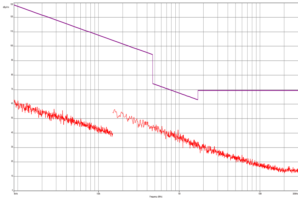
Plot 3: 9 kHz to 30 MHz, RX mode
