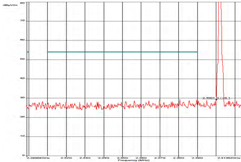
Plot 1: Lower band edge, 8 DPSK modulation, vertical & horizontal polarization
