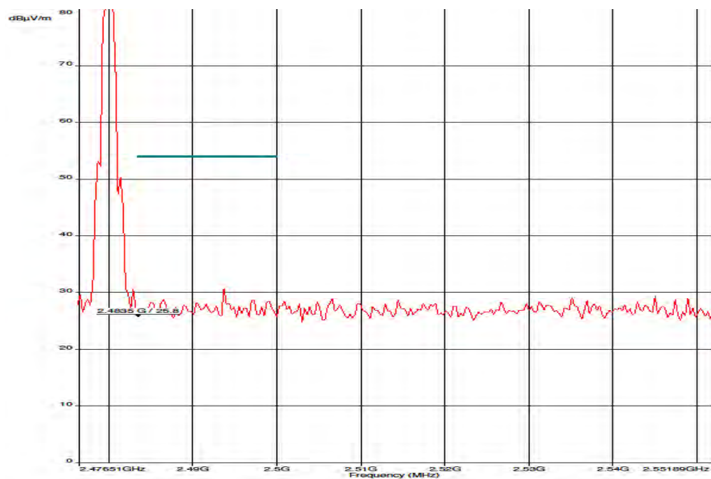
Plot 2: Upper band edge, 8 DPSK modulation, vertical & horizontal polarization
