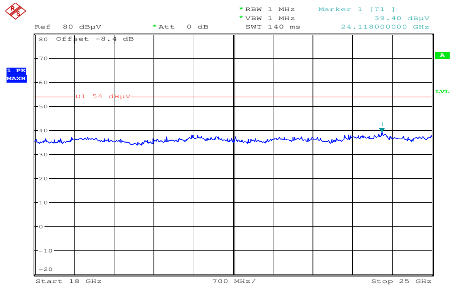
Plot 12: 18 GHz to 25 GHz, TX mode, channel 78, vertical & horizontal polarization
