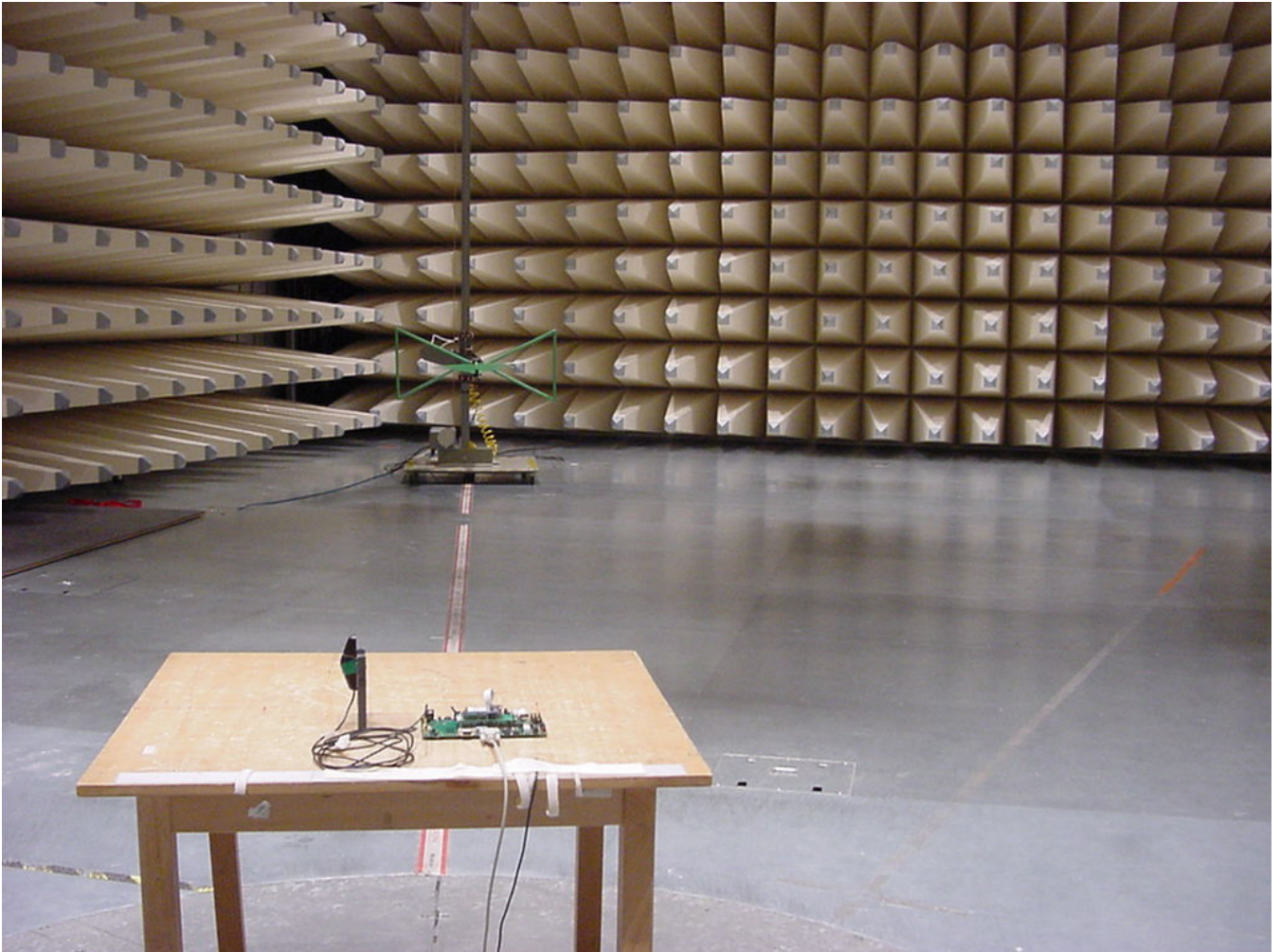
Photo 7 (Radiated Emissions):
