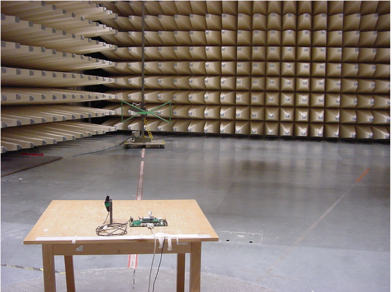
Photo 7 (Radiated Emissions):
