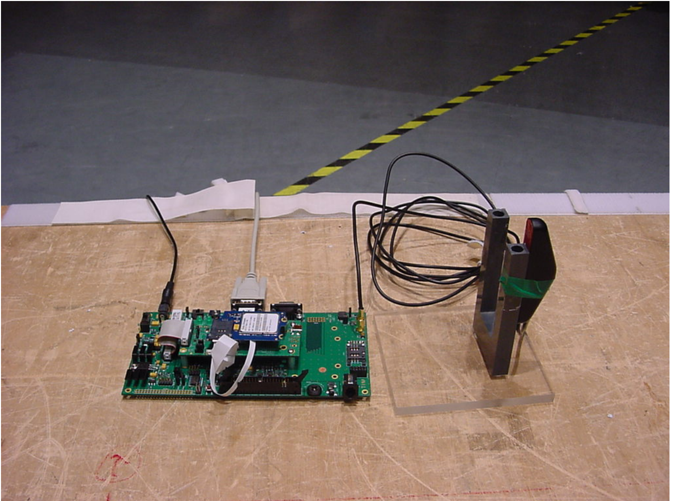
Photo 8 (Radiated Emissions):
