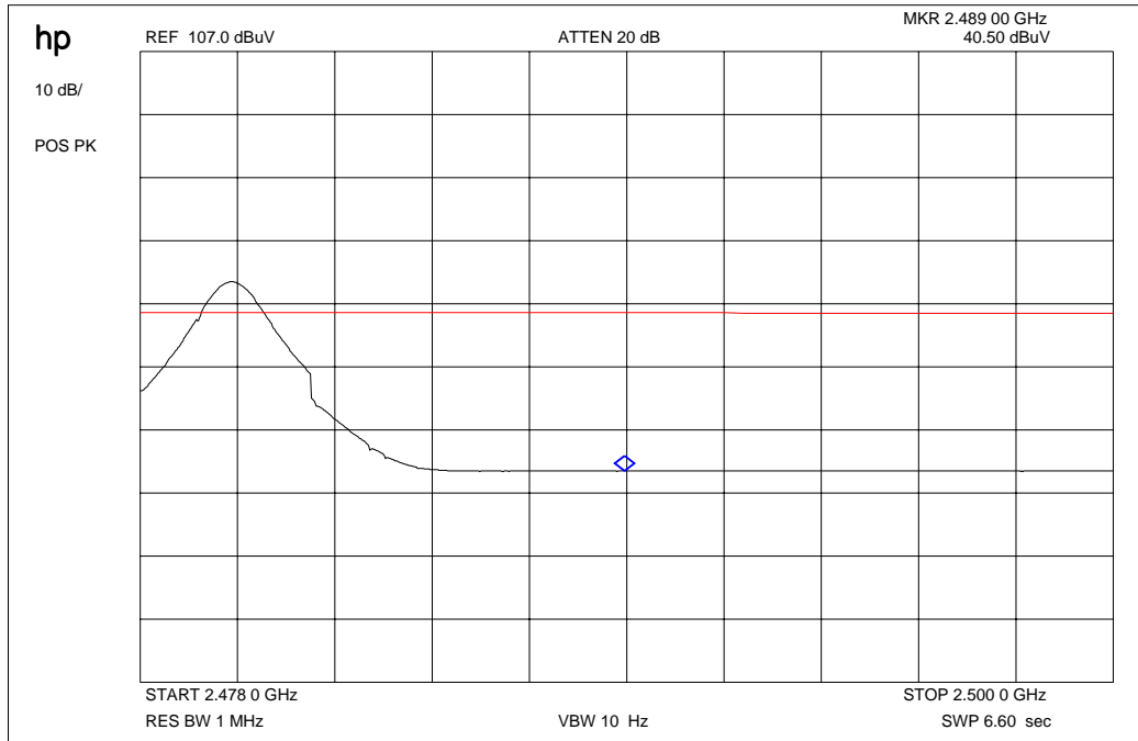
Plot 5: Restricted Bands high
