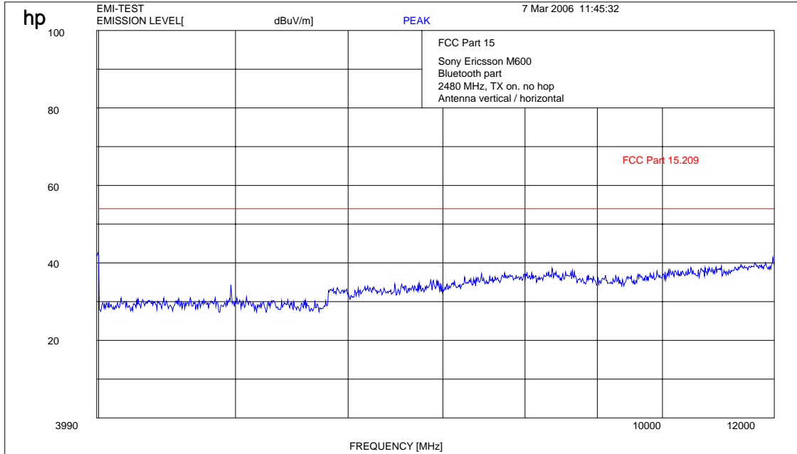
Plot : 4- 12 GHz vertical/horizontal (highest channel)
