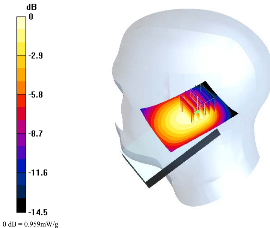
(d) Distribution of SAR in the GSM850 mode giving the maximum 1g SAR in the right hand side phantom for the tilt position
