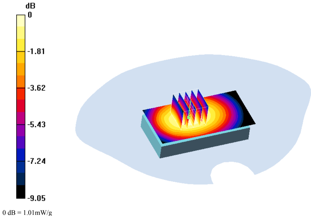
(e) Distribution of maximum SAR in GSM850 mode with muscle tissue simulating liquid giving the maximum 1g and 10g averaged SAR. Measured against the flat section of the phantom with the back of the device facing the phantom and with a 15 mm separation between the device and the liquid.
