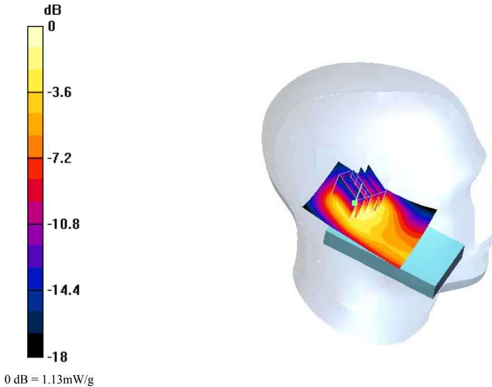
(g) Distribution of SAR in the GSM1900 mode giving the maximum 1g SAR in the left hand side phantom for the cheek position
