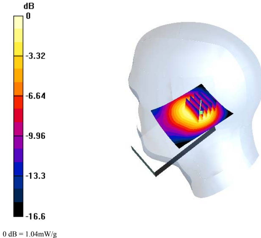
(j) Distribution of SAR in the GSM1900 mode giving the maximum 1g SAR in the right hand side phantom for the tilt position
