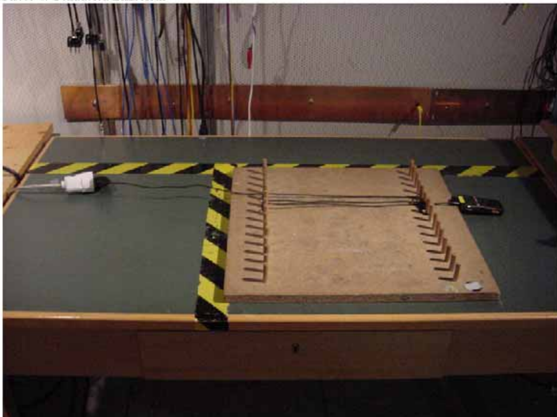
Photo 4: Conducted Emissions setup
