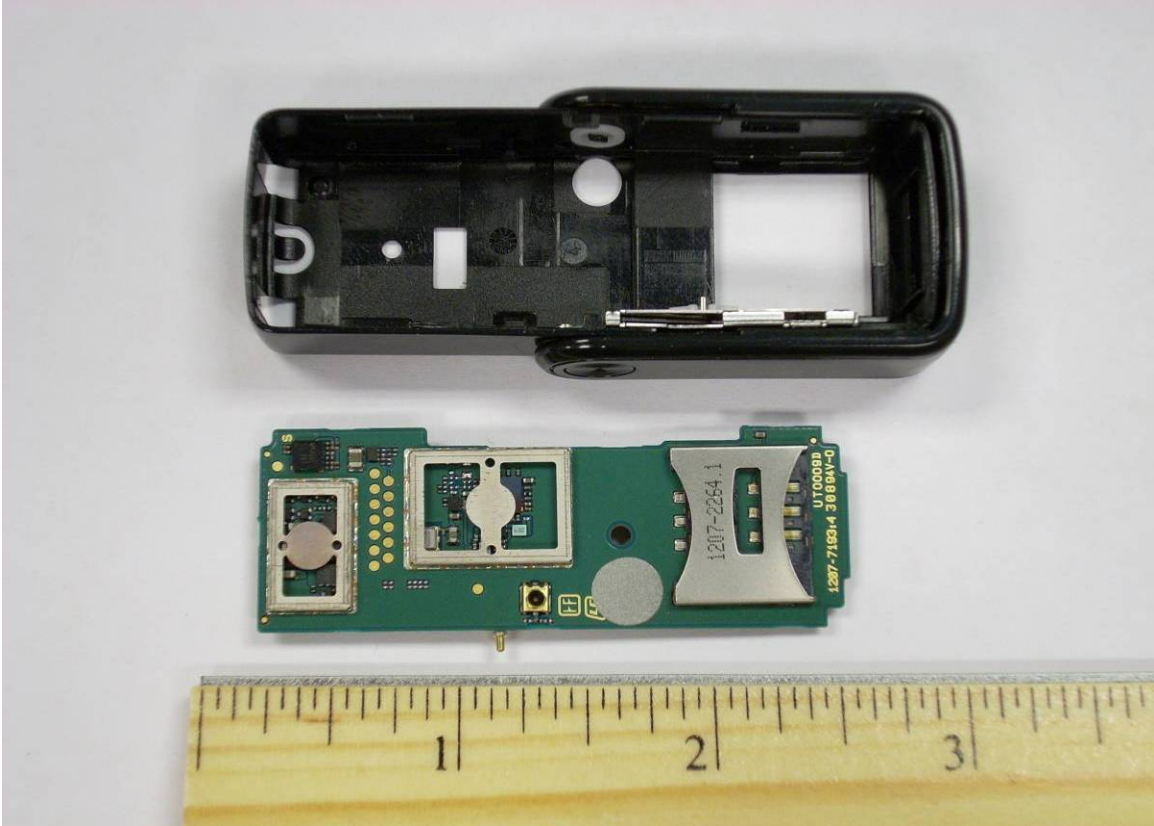
PCB Board 3 w/o Shield Cans
