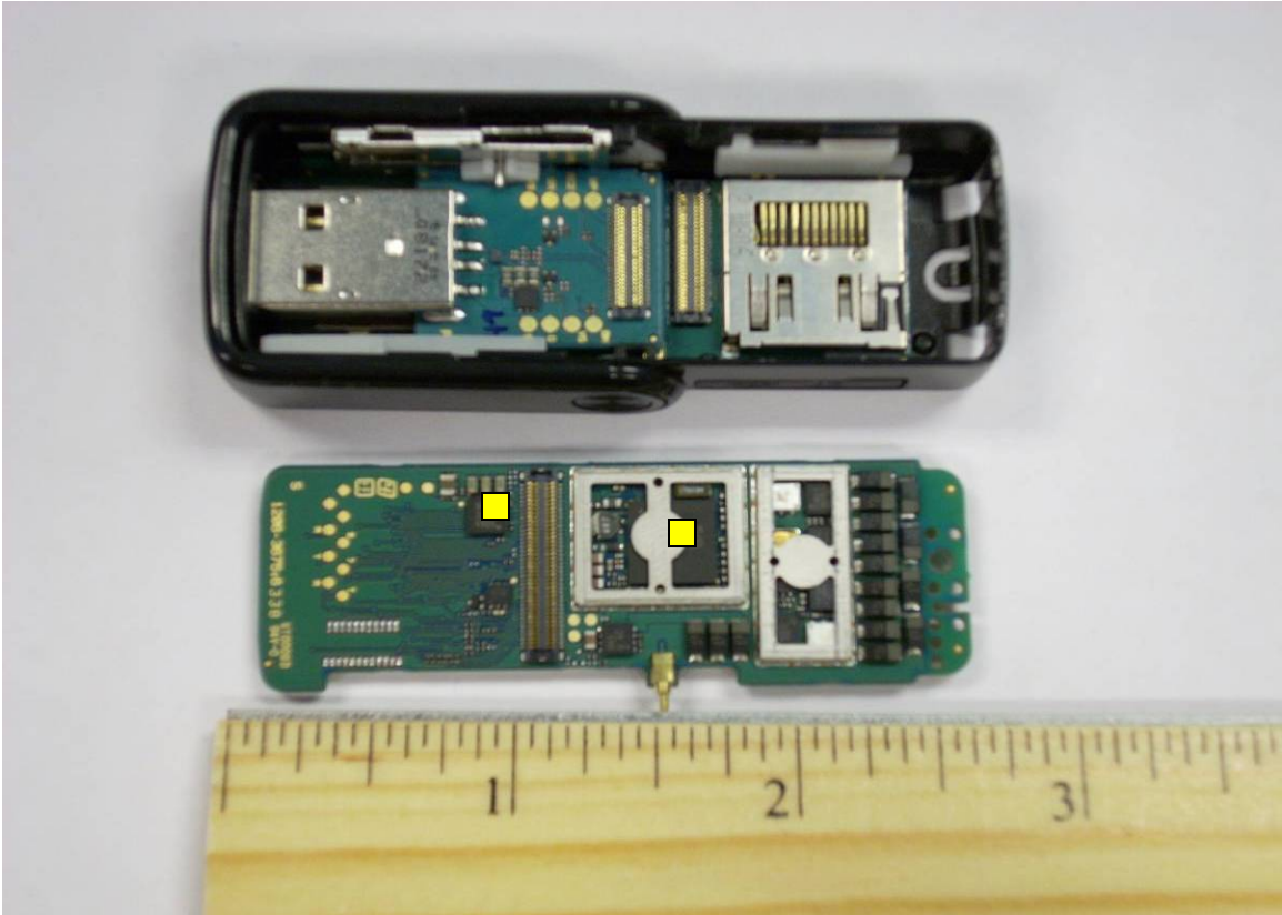
PCB Board 1 w/flex ribbon cable removed and shield cans removed
