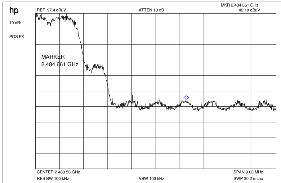
Plot 8: \pi/4 DQPSK / Marker-Delta Method (hopping)
