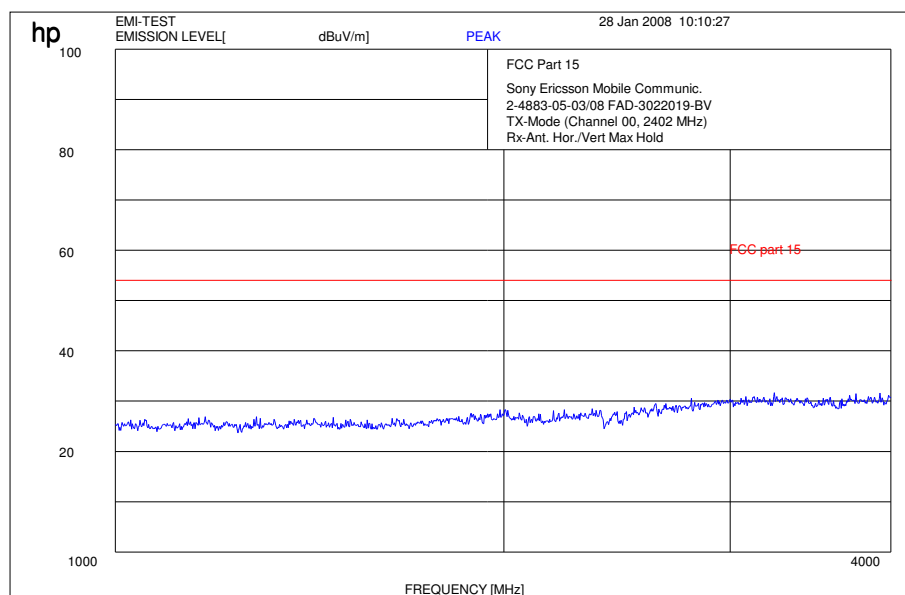
Plot: 1 - 4 GHz vertical/horizontal (lowest channel)
