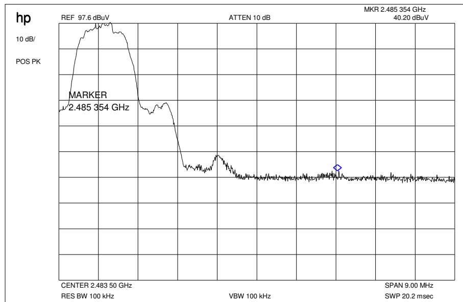
Plot 12: 8DPSK / Marker-Delta Method (single carrier)
