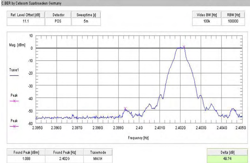
Plot 1 (GFSK, hopping off, lower band-edge):
