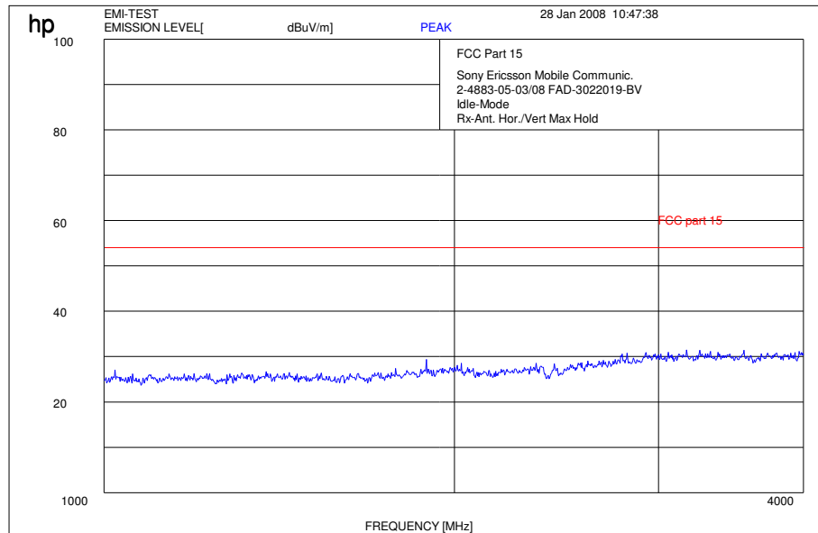
Plot: 1 - 4 GHz vertical/horizontal (receiver)
