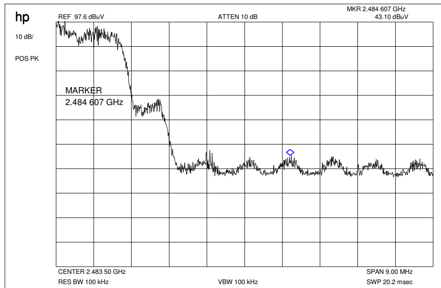
Plot 13: 8DPSK / Marker-Delta Method (hopping)
