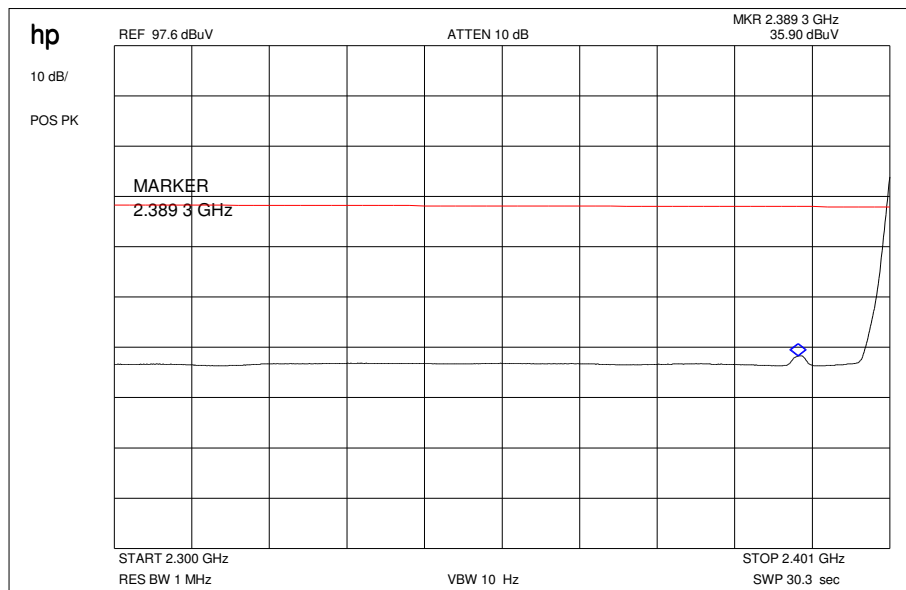
Plot 9: \pi/4 DQPSK / Restricted Bands low
