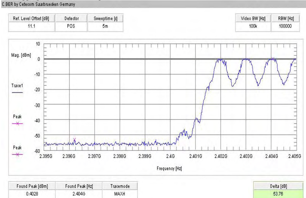
Plot 2 (GFSK, hopping on, lower band-edge):
