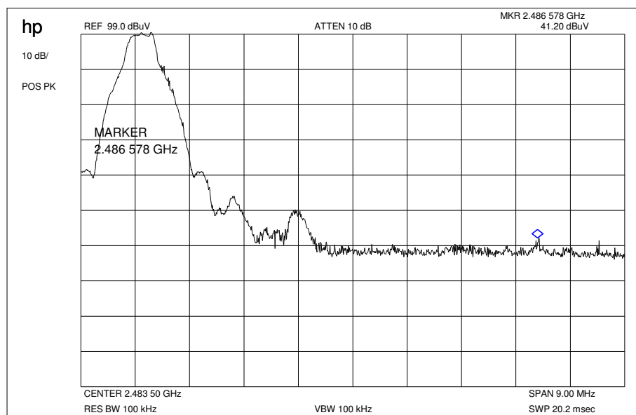
Plot 2: GFSK / Marker-Delta Method (single carrier)
