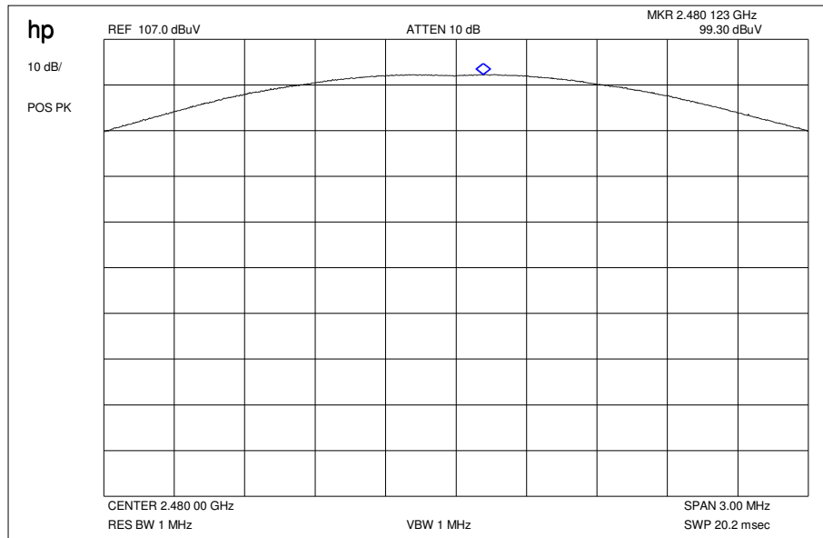
Plot 6: \pi/4 DQPSK / Max field strength in 3m distance (single frequency)
