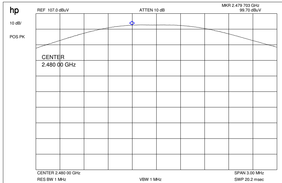
Plot 1: GFSK / Max field strength in 3m distance (single frequency)
