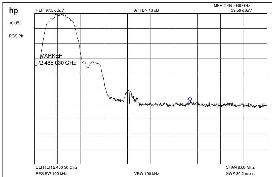
Plot 7: \pi/4 DQPSK / Marker-Delta Method (single carrier)
