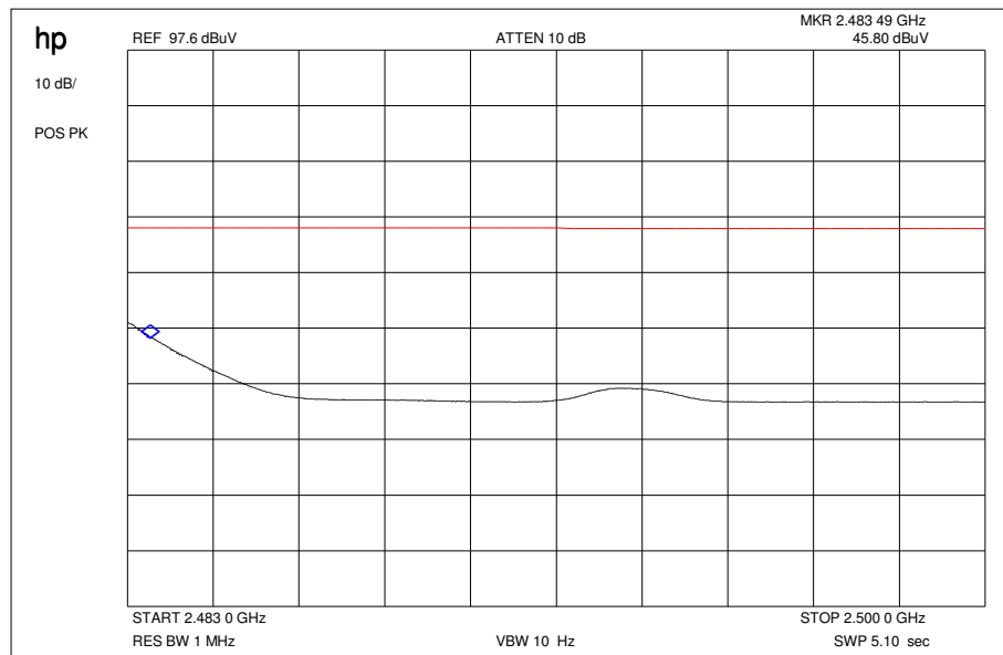
Plot 10: \pi/4 DQPSK / Restricted Bands high
