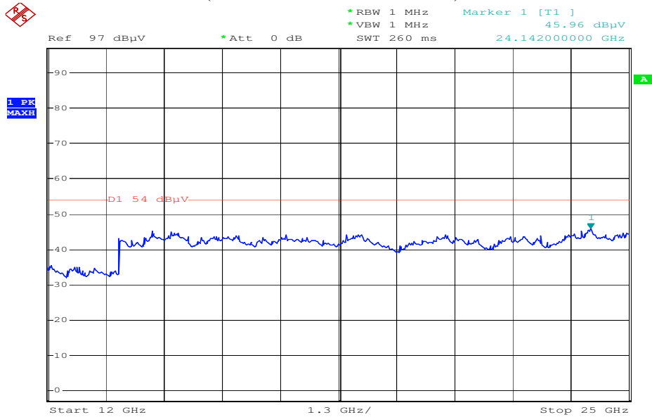
Plot: 12 - 25 GHz vertical/horizontal (valid for all channels and modes)
