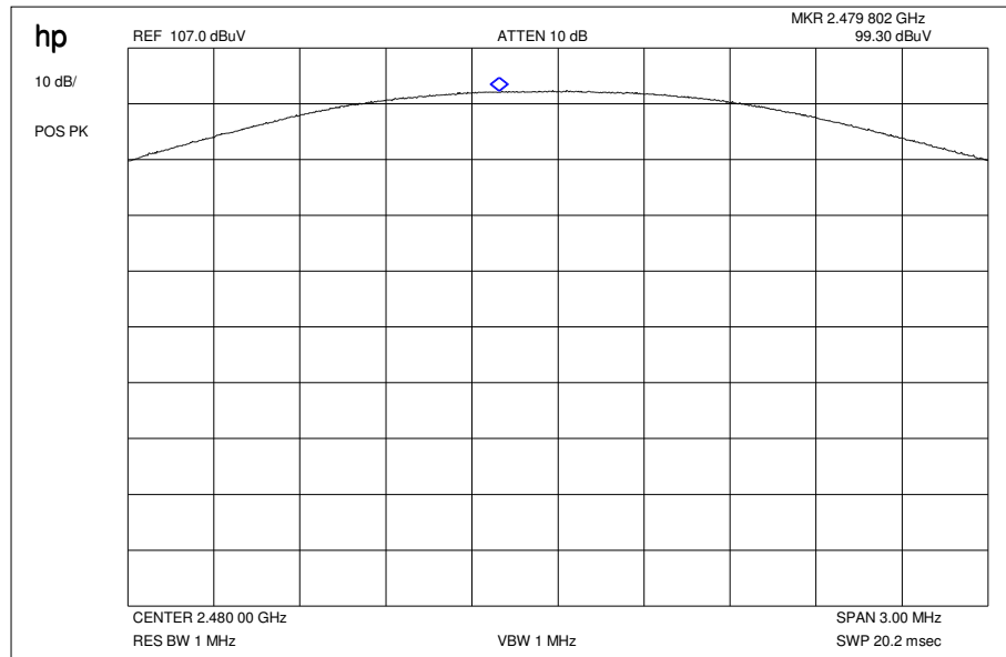
Plot 11: 8DPSK / Max field strength in 3m distance (single frequency)
