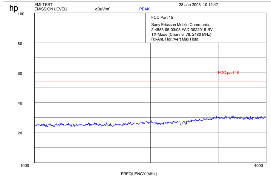
Carrier suppressed with a rejection filter
