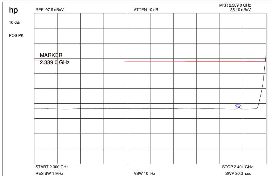
Plot 4: GFSK / Restricted Bands low
