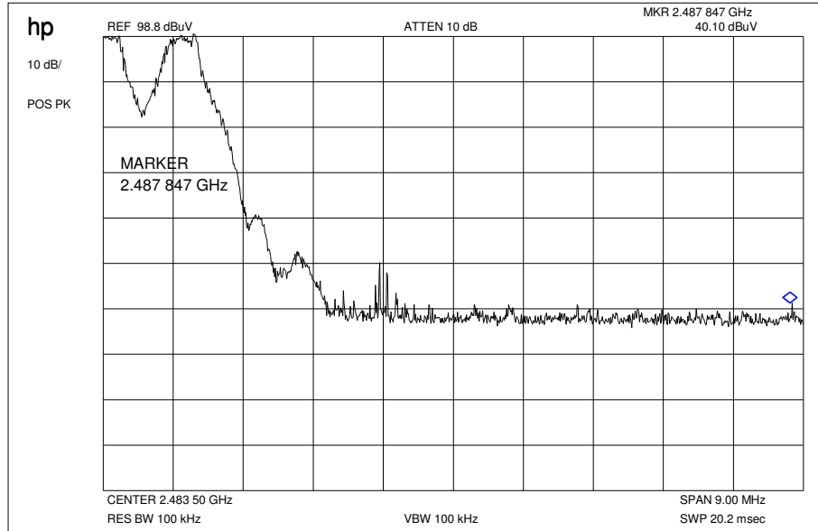
Plot 3: GFSK / Marker-Delta Method (hopping)
