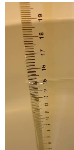
Measured level (151 mm, flat section) of 2450 MHz muscle tissue simulating liquid in phantom
