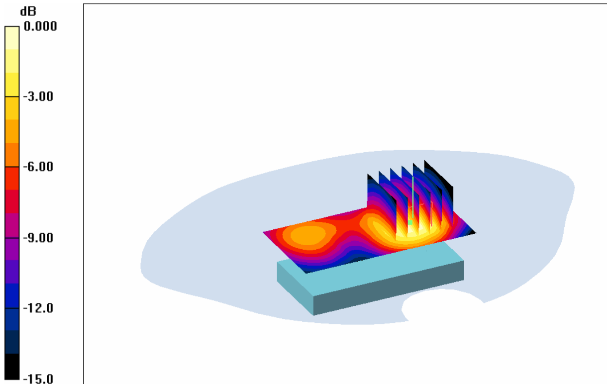
(e) Maximum SAR Distribution for EUT in GSM1900 mode measured with the back of the phone facing the flat section of phantom.
