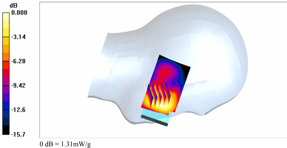
(c) SAR Distribution for EUT in GSM1900 mode measured against the left hand side phantom for the cheek phone position.
