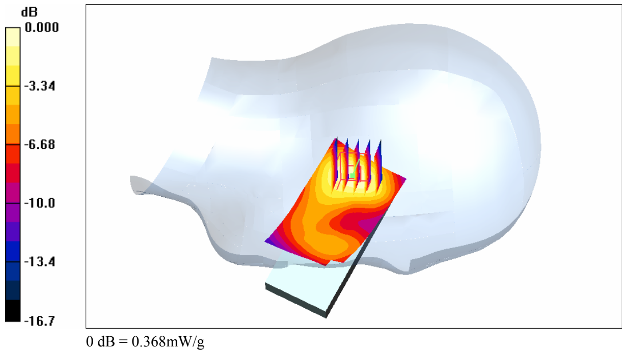
(d) SAR Distribution for EUT in GSM1900 mode measured against the left hand side phantom for the tilt phone position.
