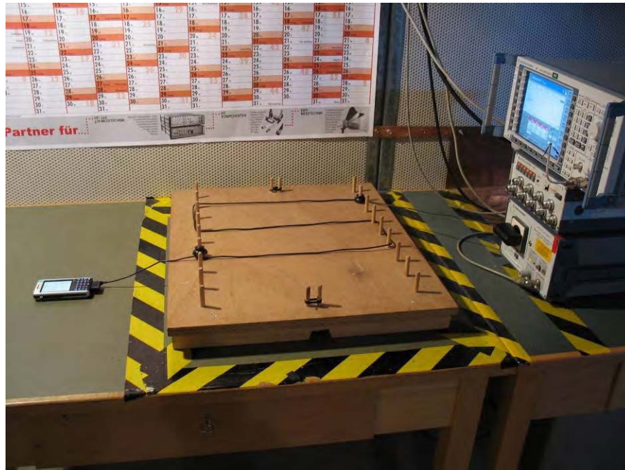
Photo 3: Conducted Emissions
