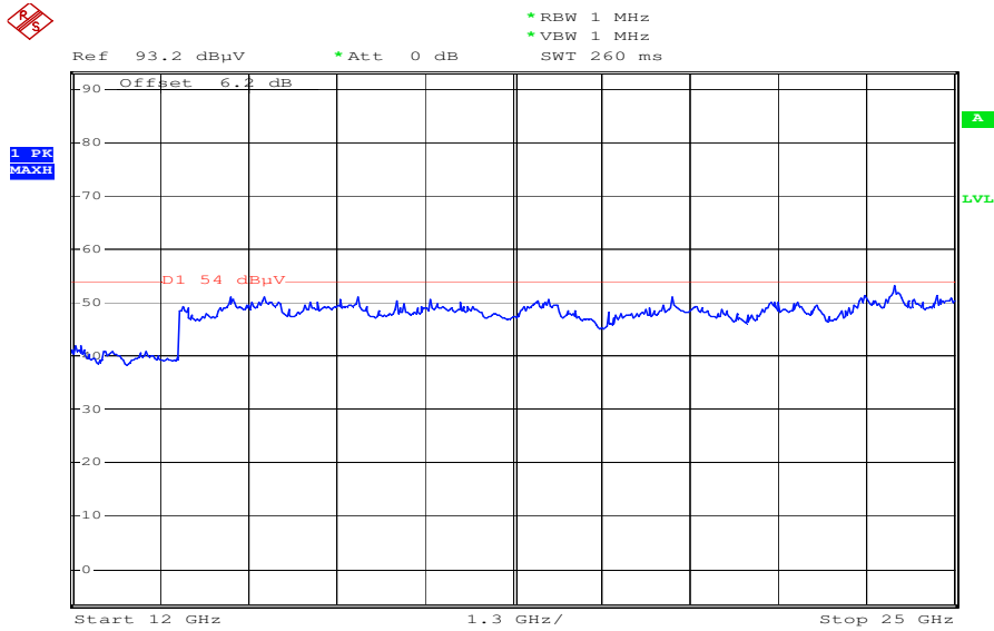
Plot : 12- 25 GHz vertical worst case (valid for all three channels)
