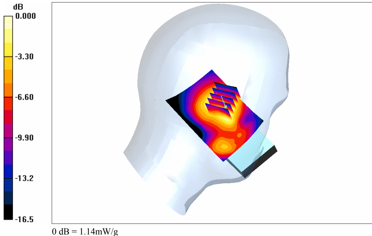
(c) Maximum SAR Distribution for EUT in GSM1900 mode measured against the left hand side phantom for the cheek phone position.
