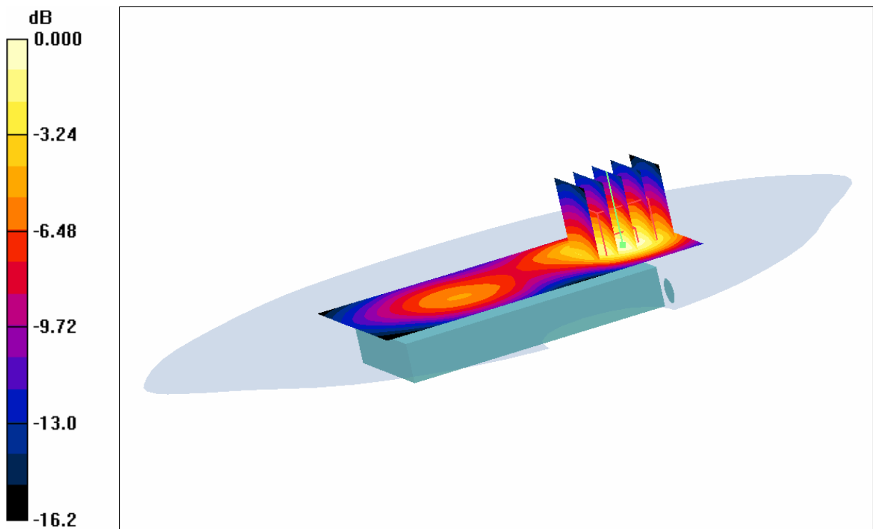
(f) Maximum SAR Distribution for EUT in GPRS(2Tx)1900 mode measured with the back of the phone facing the flat section of phantom.
