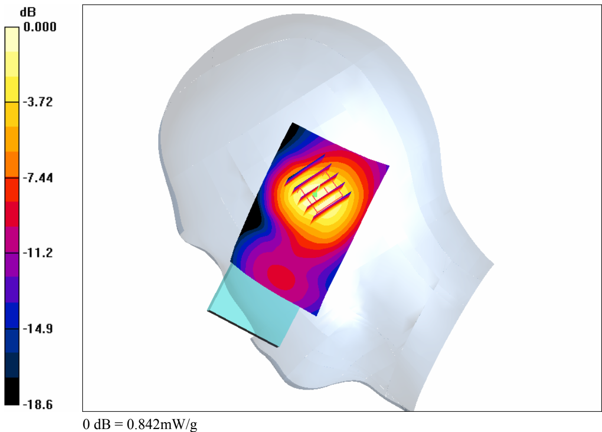
(b) SAR Distribution for EUT in GSM1900 mode measured against the right hand side phantom for the tilt phone position.
