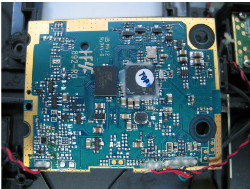
Photo 4: PCB top view
