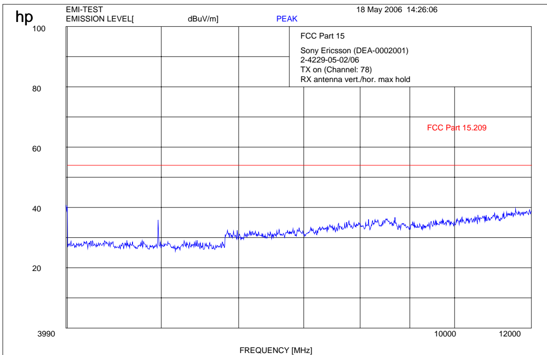
Plot : 4- 12 GHz vertical/horizontal (highest channel)
