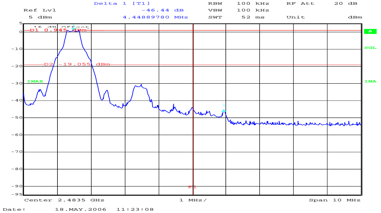
Plot 3 of 4 (hopping off, highest frequency):
