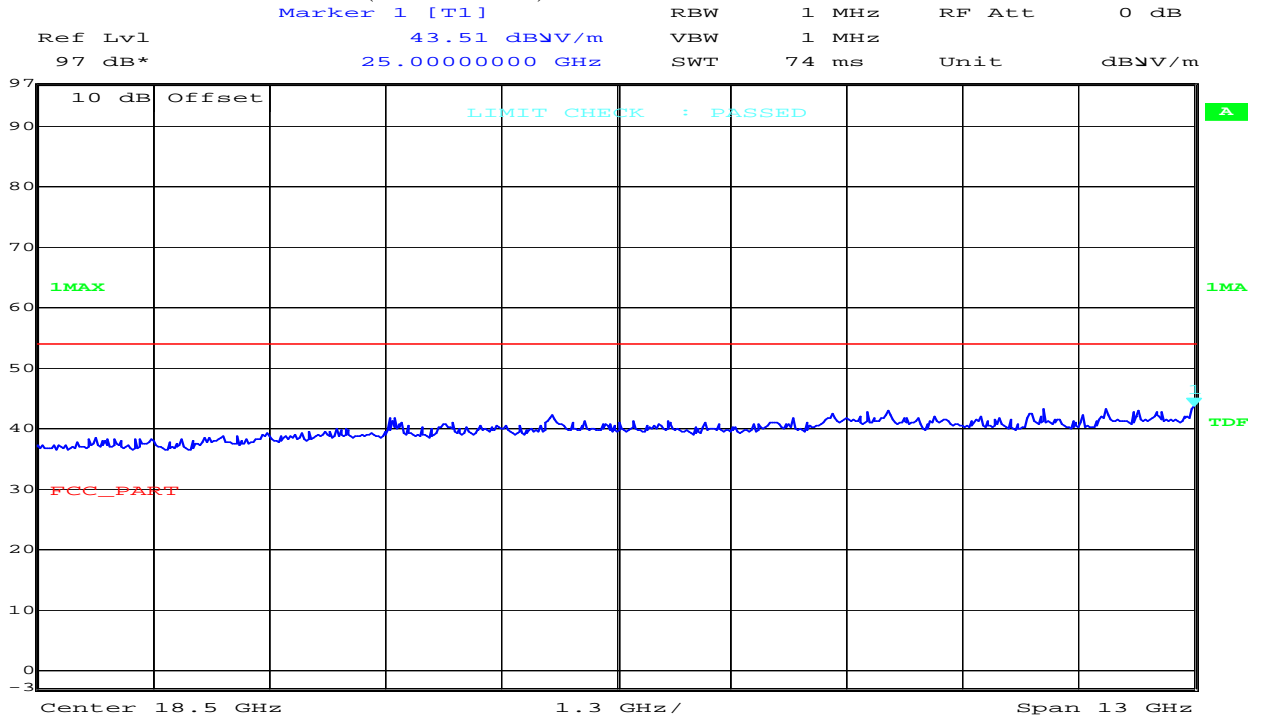
Plot : 12- 25 GHz vertical/horizontal (middle channel)
