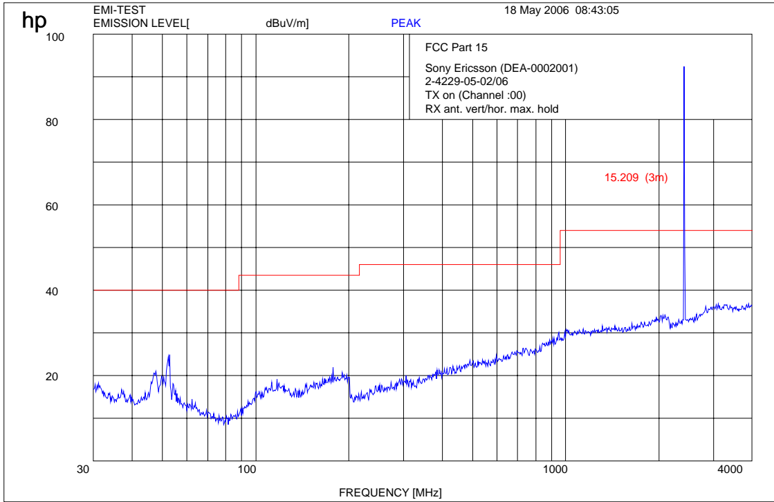
Plot : 0.03 - 4 GHz vertical/horizontal (lowest channel)
