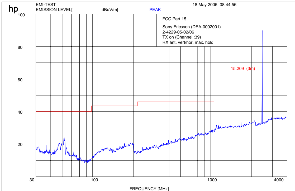
Plot : 0.03 - 4 GHz vertical/horizontal (middle channel)
