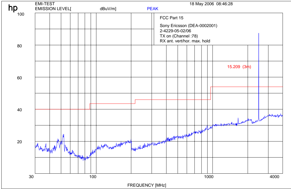
Plot : 0.03 - 4 GHz vertical/horizontal (highest channel)
