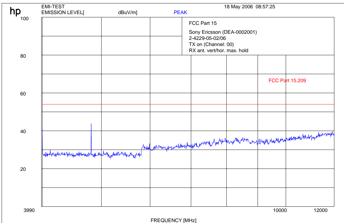
Plot : 4- 12 GHz vertical/horizontal (lowest channel)
