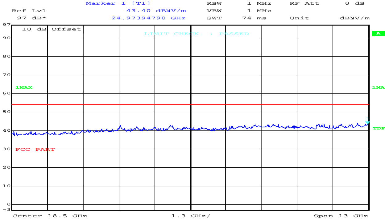
Plot : 12- 25 GHz vertical/horizontal (lowest channel)
