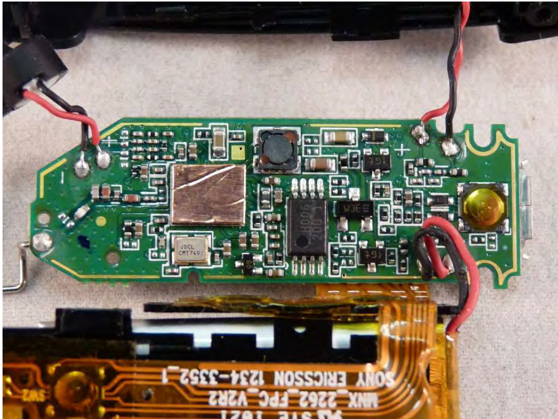
Product disassembled (PCB, Bluetooth chip with shielding, top view)
