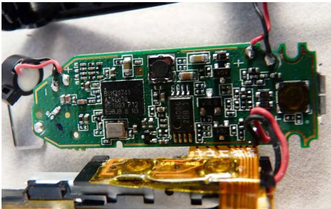
Product disassembled (PCB, Bluetooth chip w/o shielding, top view)
