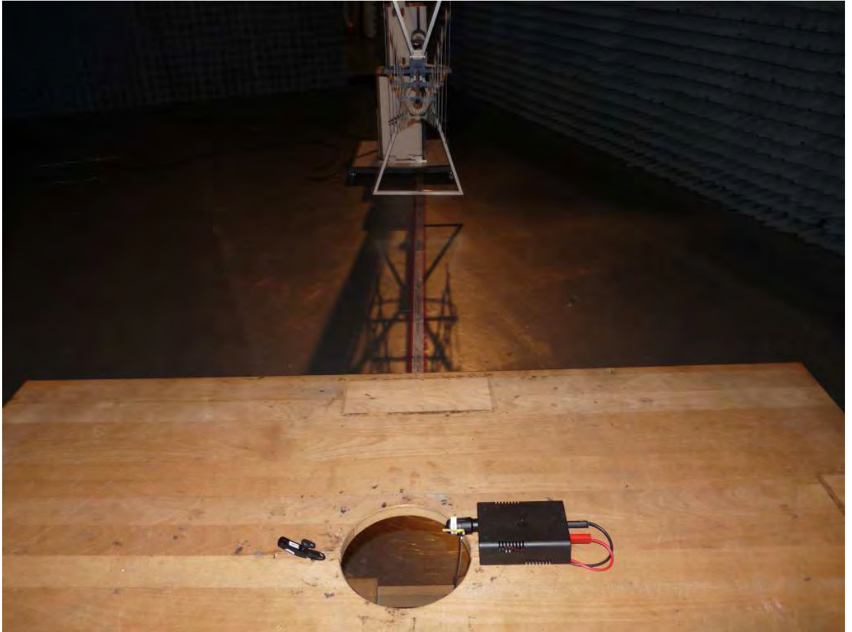
Car setup below 1GHz
