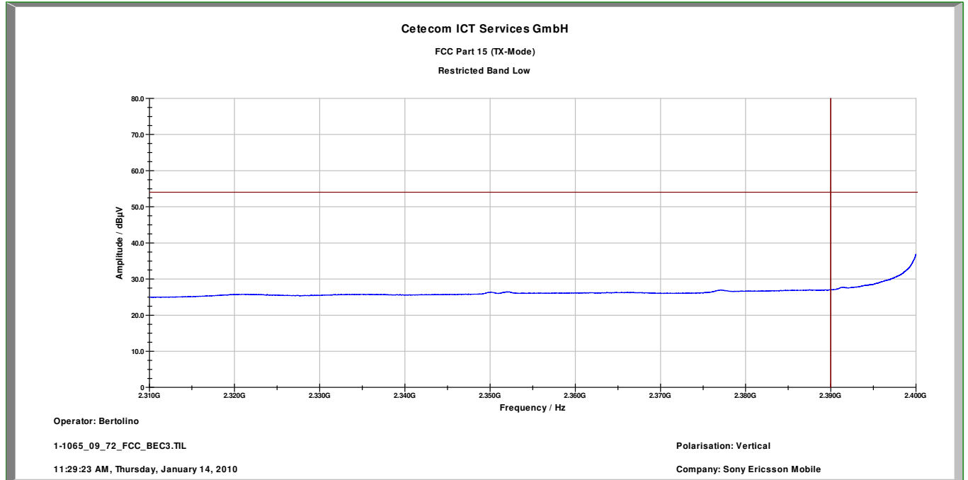
Plot 1: Restricted Bands low, vertical polarization
