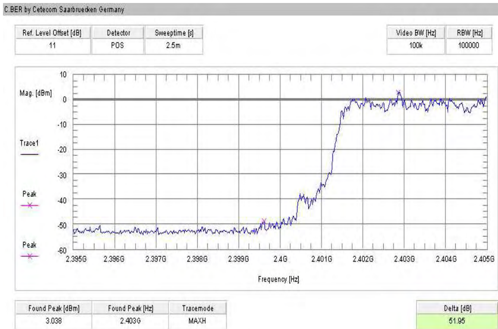
Plot 2 of 4 (hopping on, lowest frequency):
