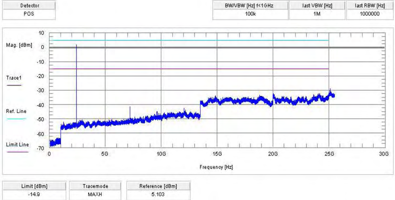
Plot 1 of 3: lowest channel
