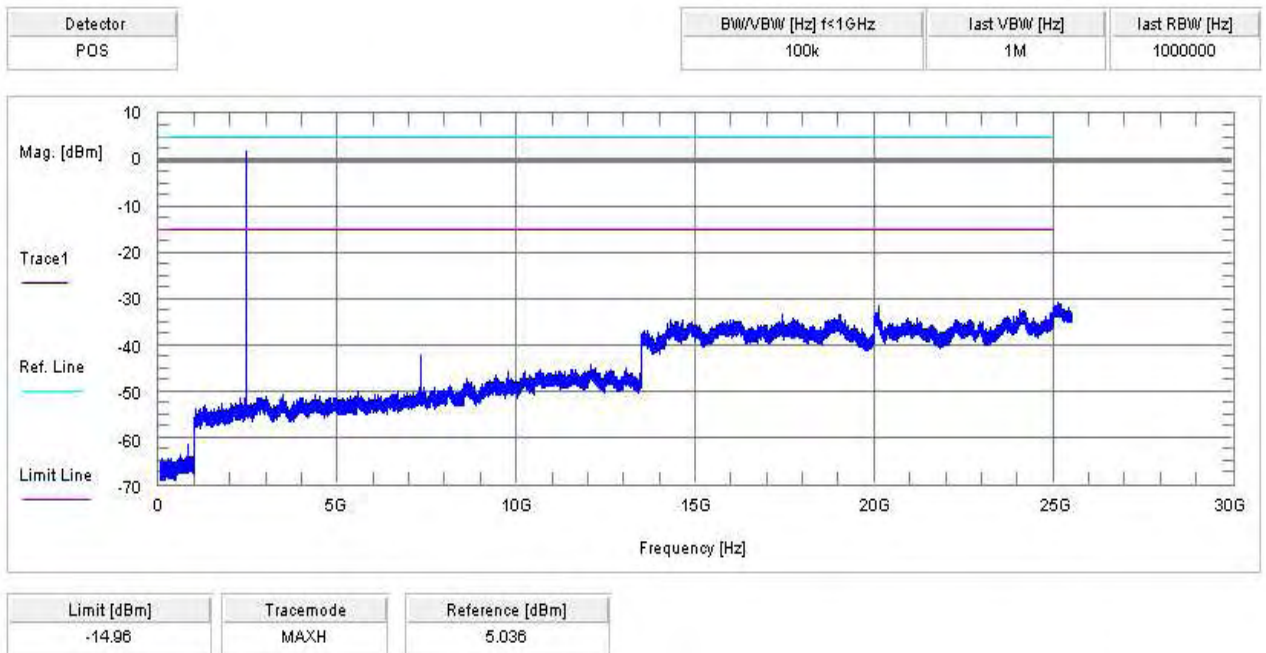
Plot 2 of 3: middle channel
