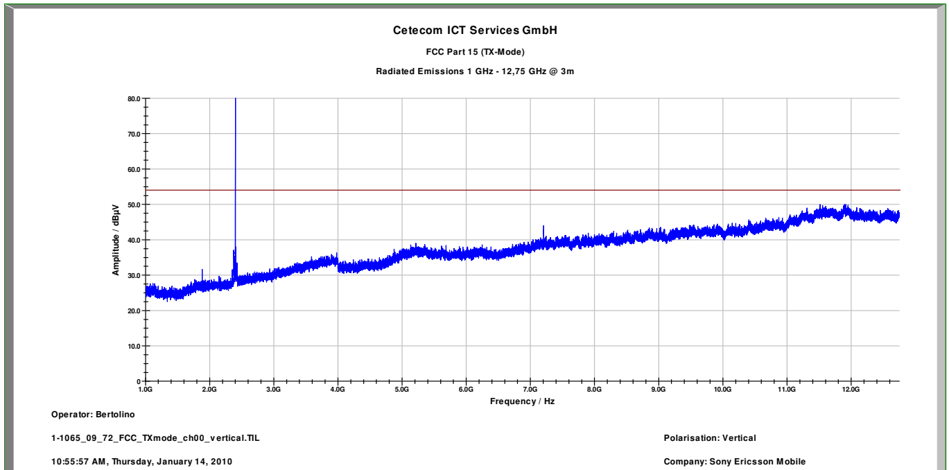
Plot 2: 1 – 12.75 GHz vertical (lowest channel)
