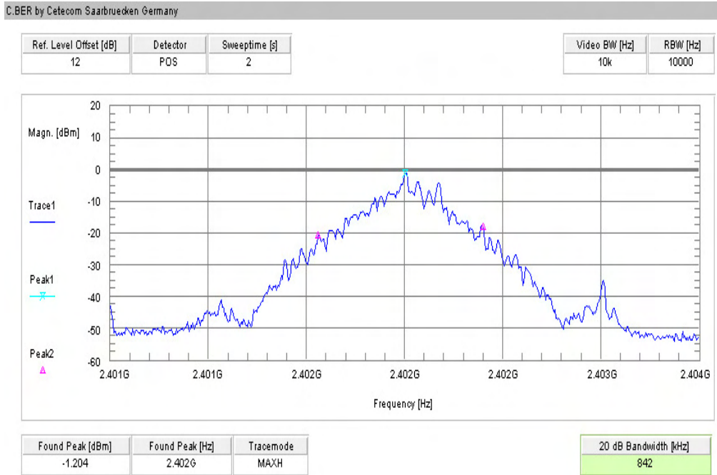
Plot 1: GFSK (Lowest channel)
