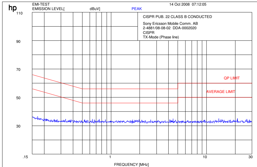
Plot 2: BT Testmode (Phase line)
