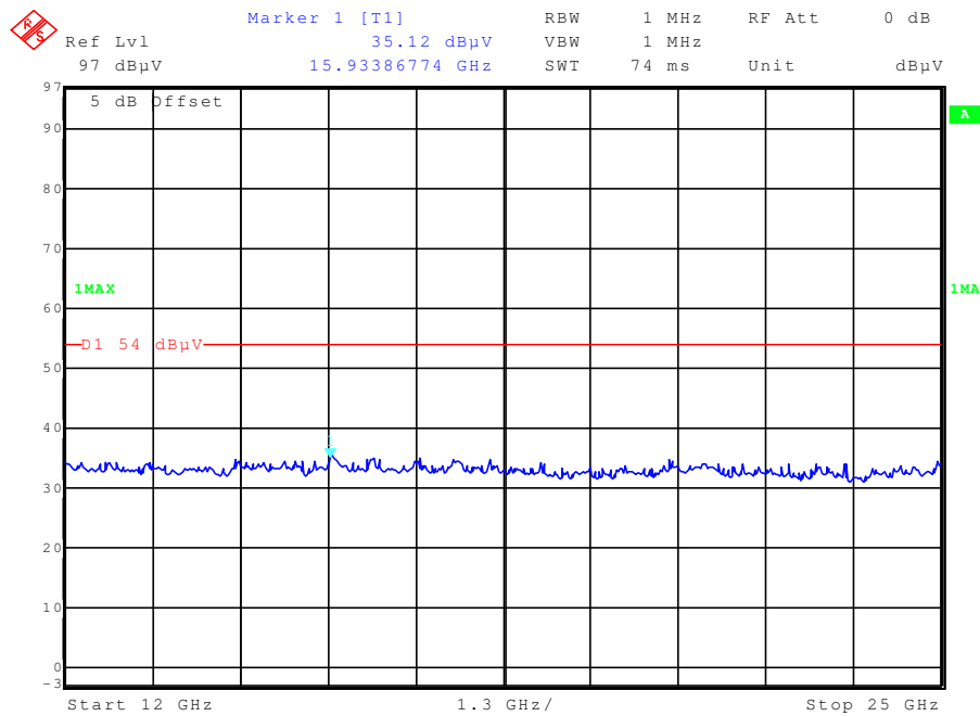
Plot 4: 12 - 25 GHz vertical/horizontal (receiver)
