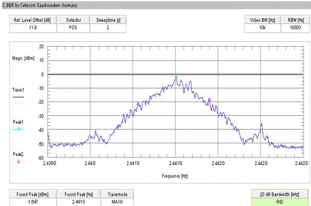
Plot 2: GFSK (Middle channel)
