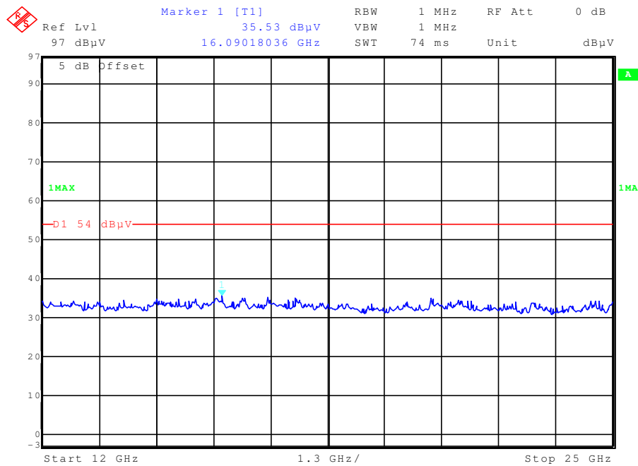
Plot 4: 12 - 25 GHz vertical/horizontal (valid for all channels)
