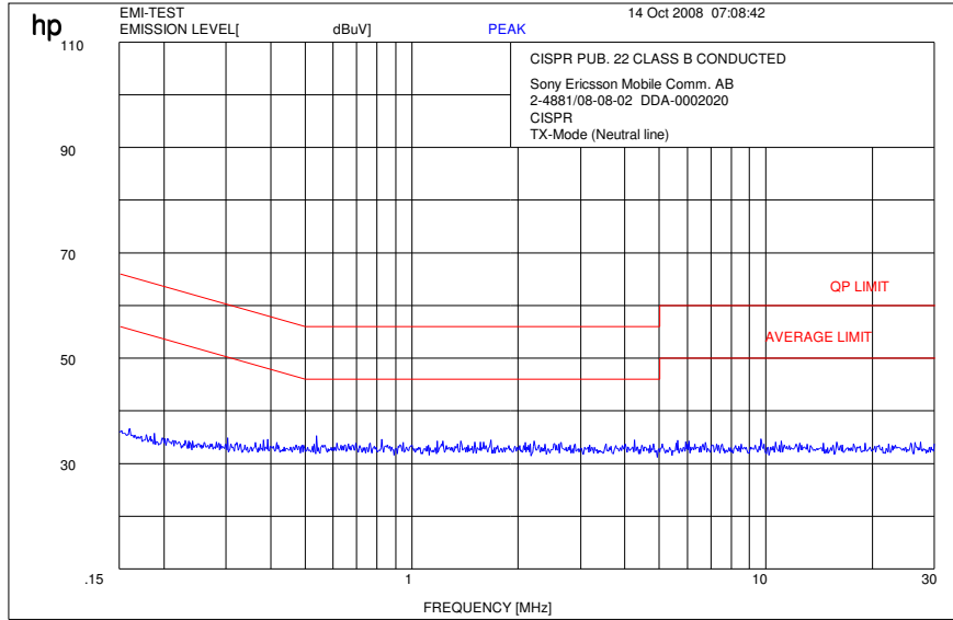
Plot 1: BT Testmode (Neutral line)
