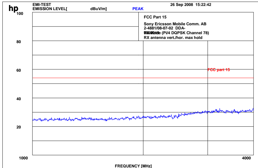
Plot 9: 1 - 4 GHz vertical/horizontal (Pi/4 DQPSK - highest channel)
