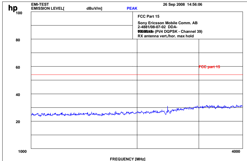
Plot 6: 1 - 4 GHz vertical/horizontal (Pi/4 DQPSK - middle channel)
