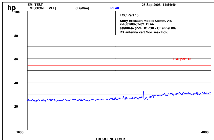
Plot 2: 1 - 4 GHz vertical/horizontal (Pi/4 DQPSK - lowest channel)
