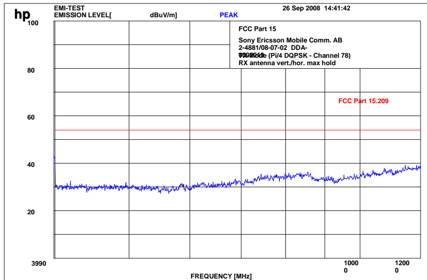
Plot 10: 4 - 12 GHz vertical/horizontal (Pi/4 DQPSK - highest channel)
