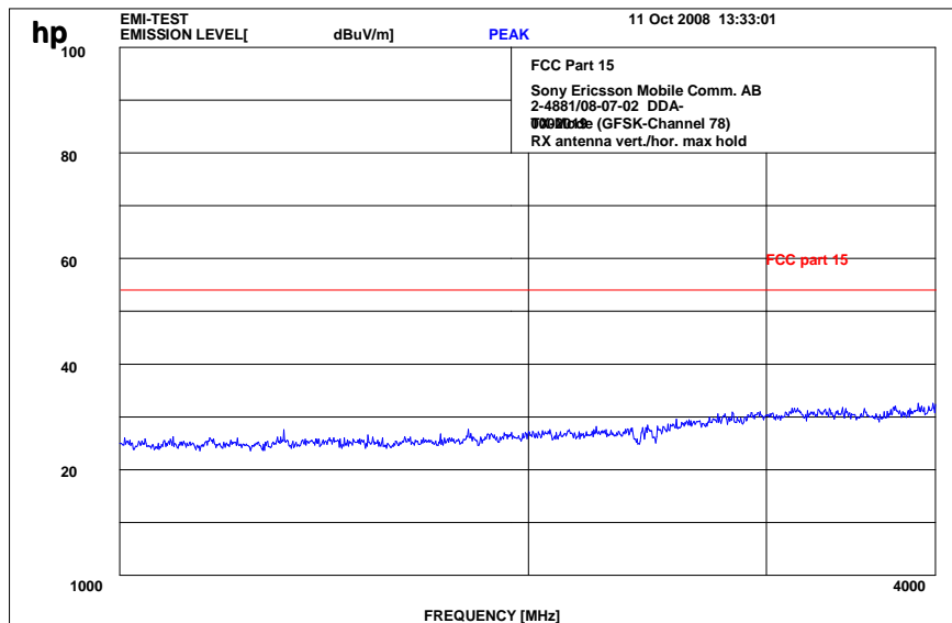
Plot 9: 1 - 4 GHz vertical/horizontal (GFSK - highest channel)
