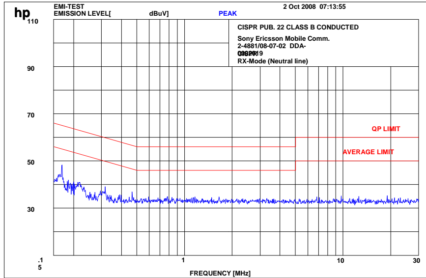
Plot 3: RX-Mode (Neutral line); valid for all modulations
