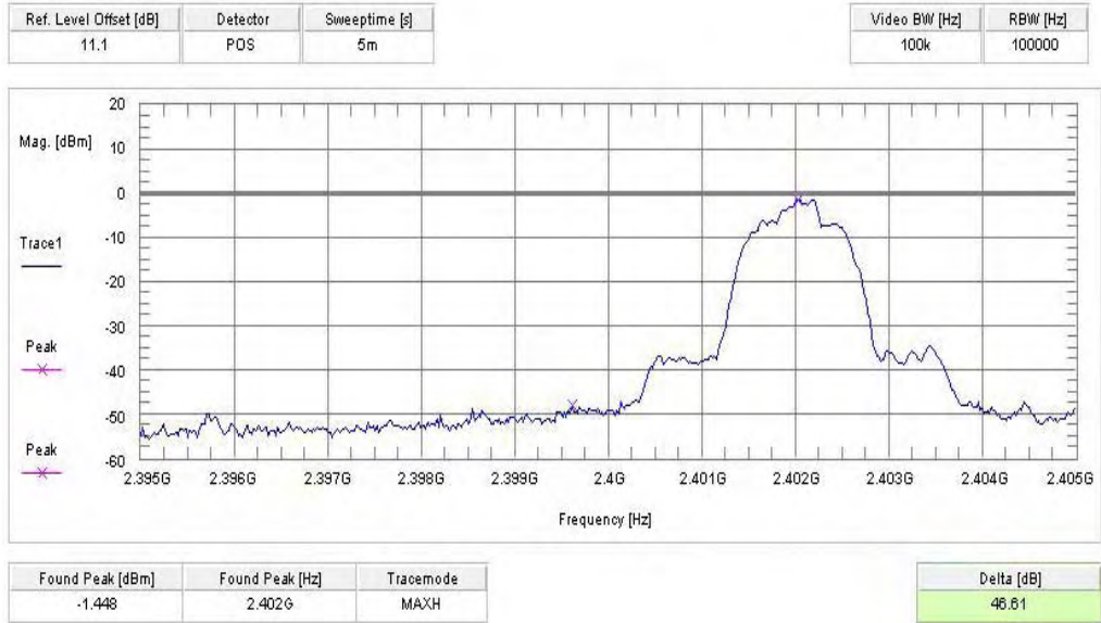
Plot 1 of 4 (hopping off, lowest frequency):
