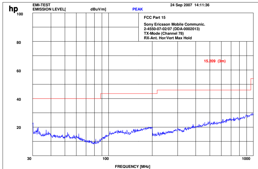
Plot: 0.03 - 1 GHz vertical/horizontal (highest channel)
