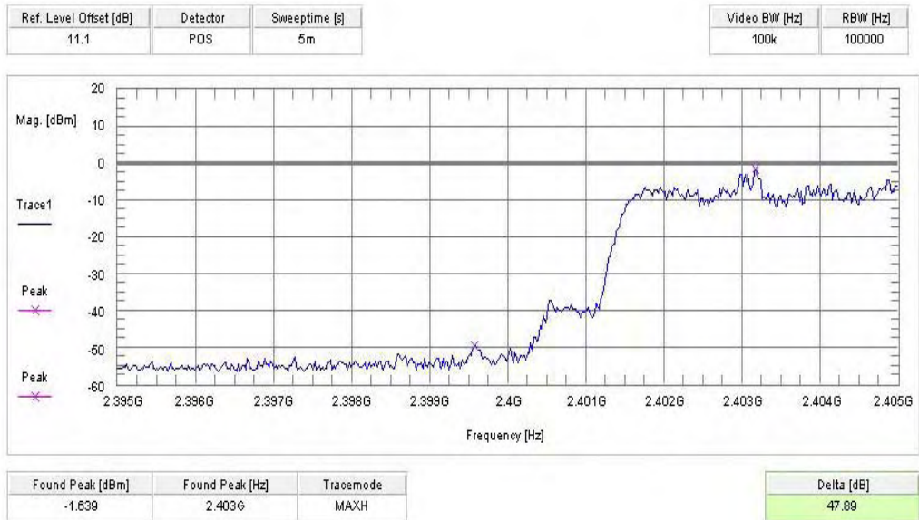
Plot 2 of 4 (hopping on, lowest frequency):
