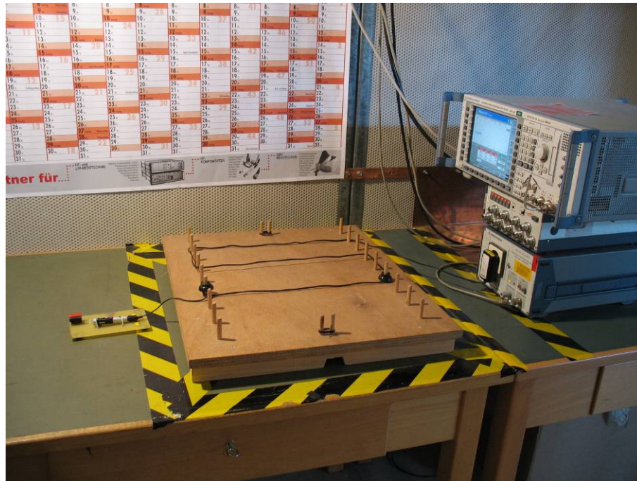
Photo 3: Conducted Emissions
