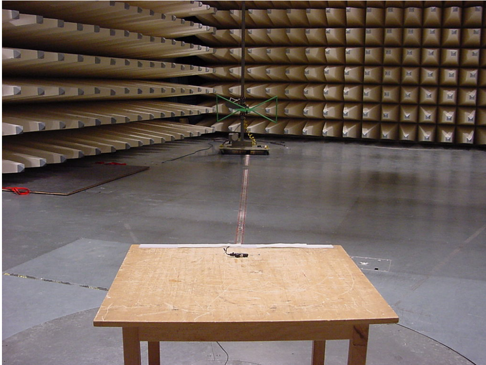
Photo 1: Radiated Emissions
