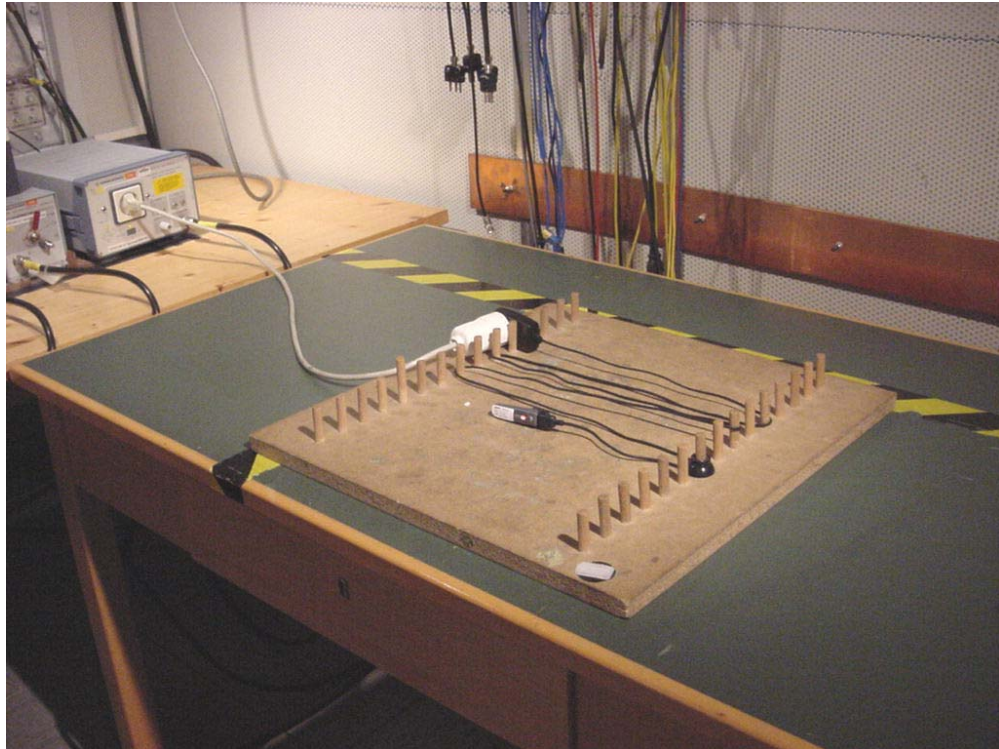
Photo 3: Conducted Emissions
