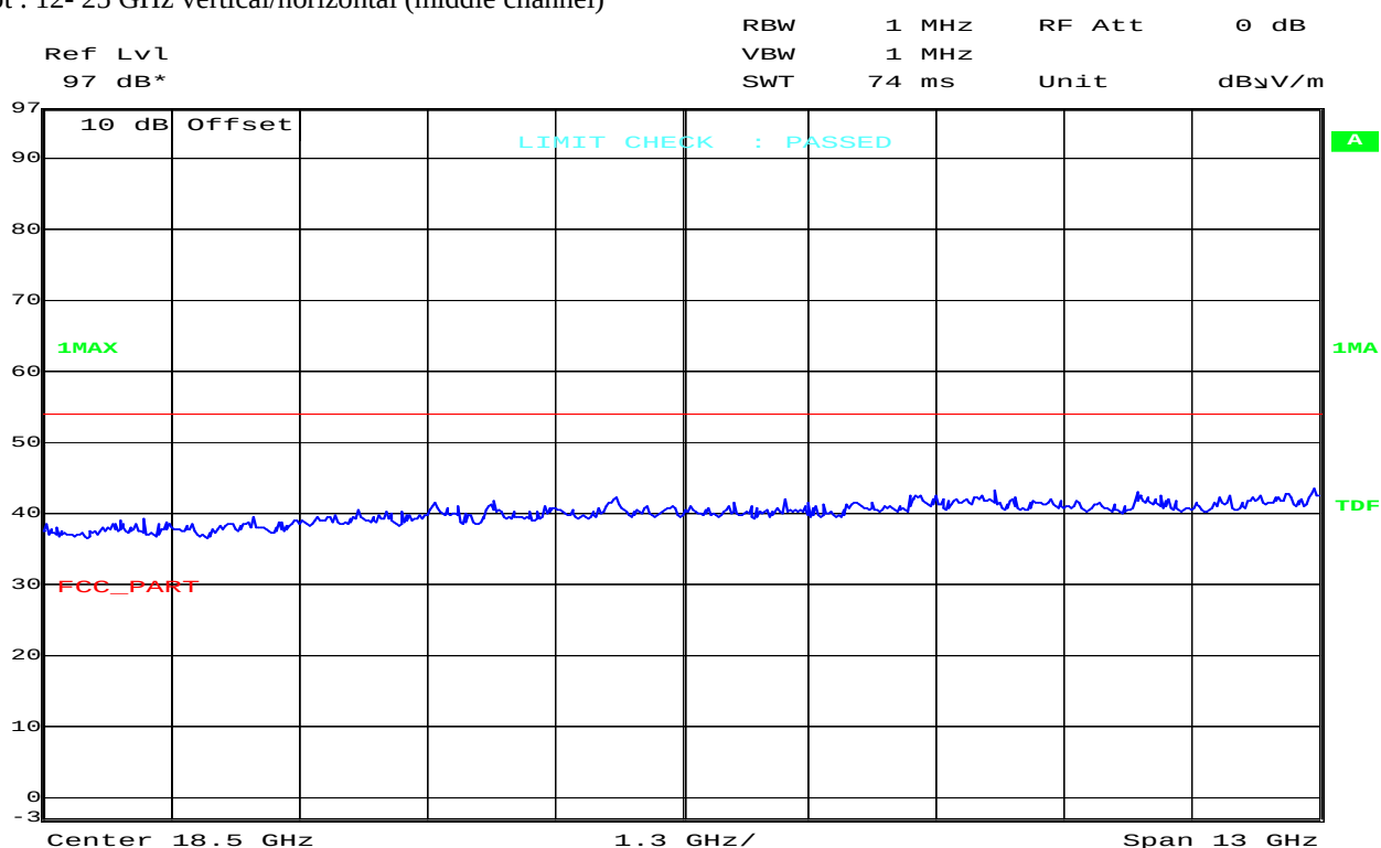
Plot : 12- 25 GHz vertical/horizontal (middle channel)
