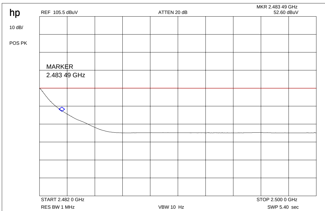
Plot 5: Restricted Bands high
