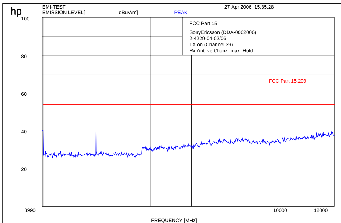
Plot : 4- 12 GHz vertical/horizontal (middle channel)
