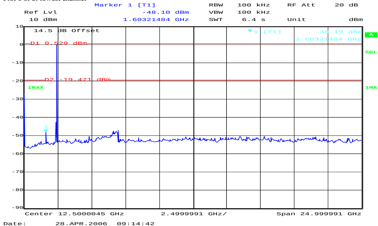
Plot 1 of 3: lowest channel
