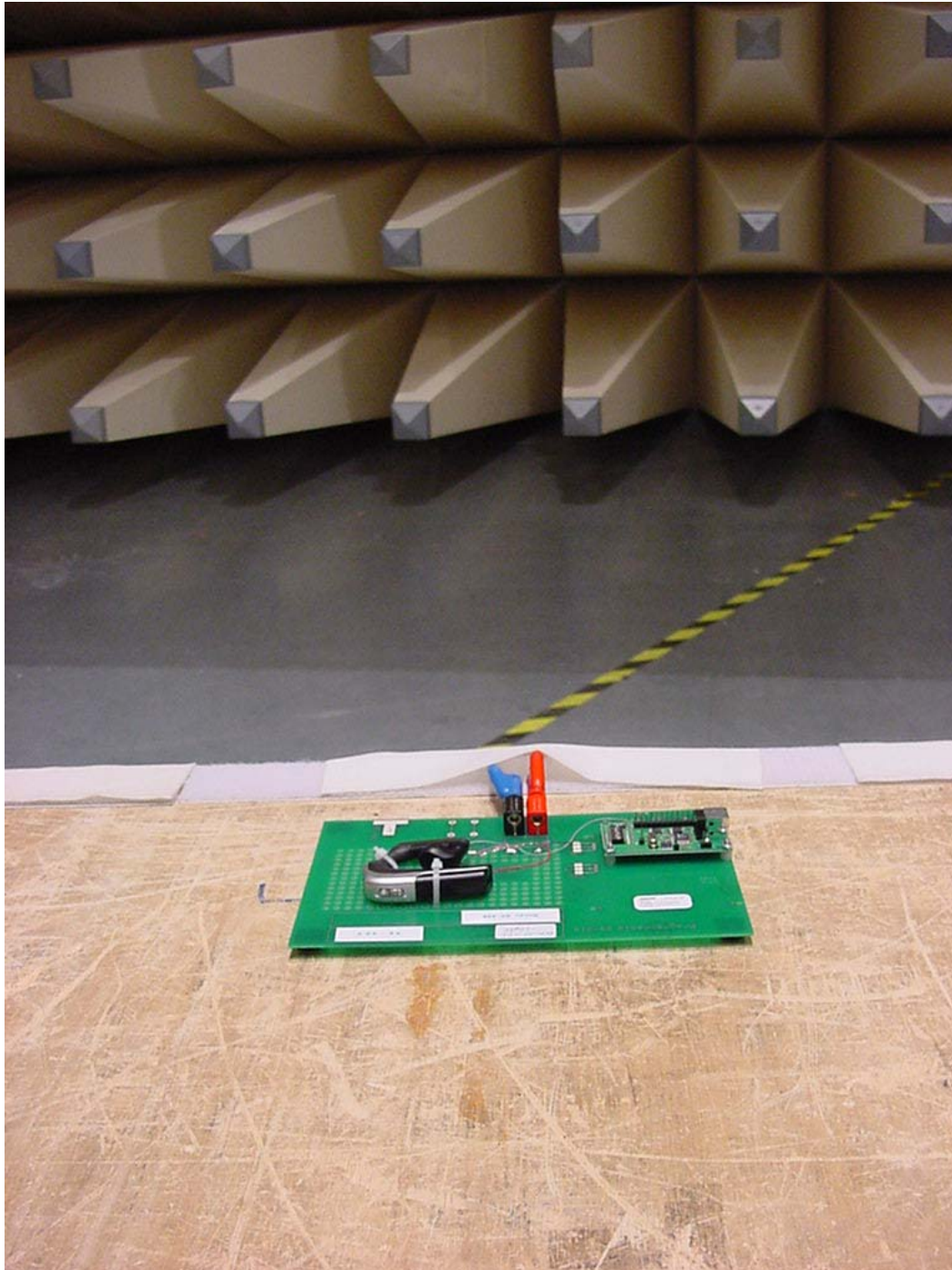
Photo 2: Radiated Emissions
