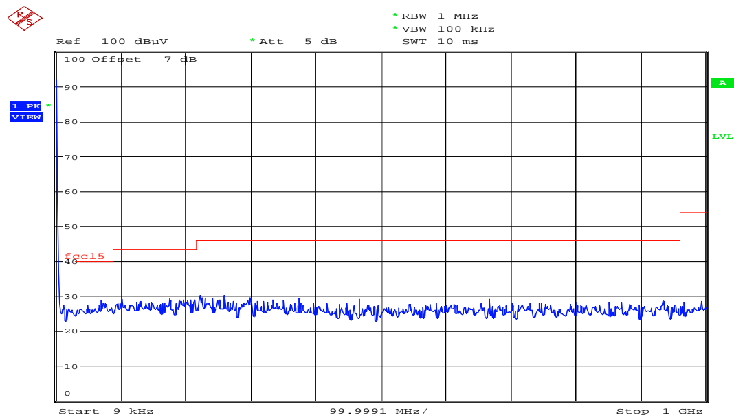
Plot 4 of 11: middle channel ( 9kHz – 1GHz)
