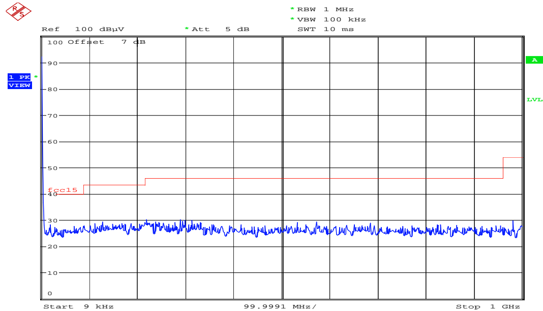
Plot 7 of 11: highest channel ( 9kHz – 1GHz)
