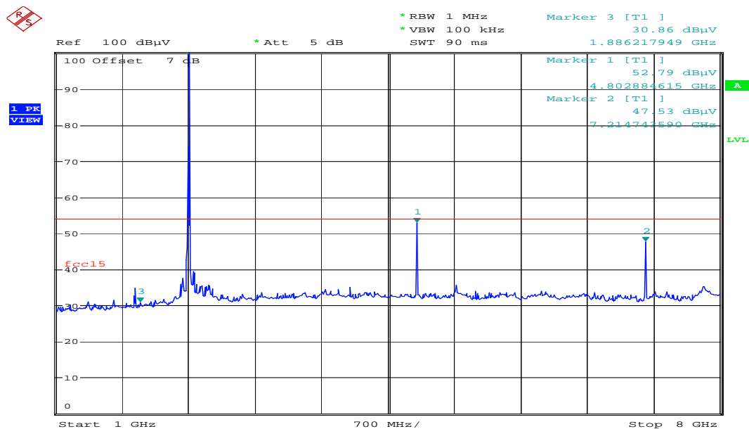
Plot 2 of 11: lowest channel ( 1GHz – 8GHz)
