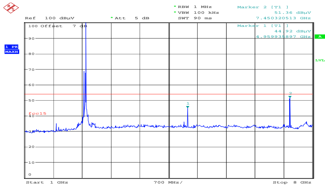
Plot 8 of 11: highest channel ( 1GHz – 8GHz)
