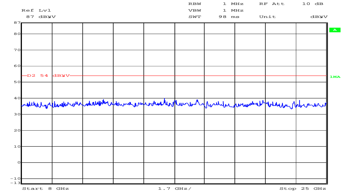
Plot 6 of 11: middle channel ( 8GHz – 25GHz)
