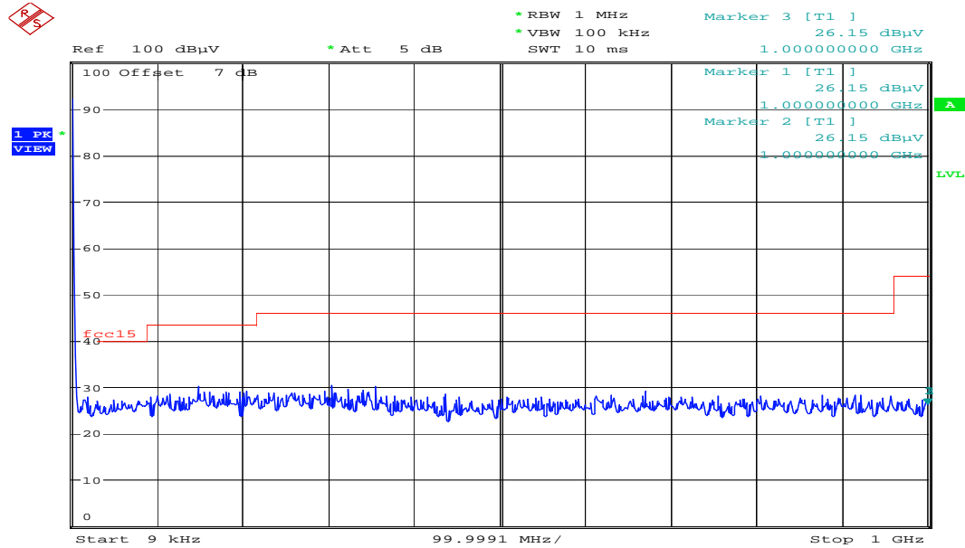
Plot 1 of 11: lowest channel ( 9kHz – 1GHz)
