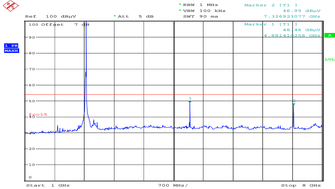
Plot 5 of 11: middle channel ( 1GHz – 8GHz)
