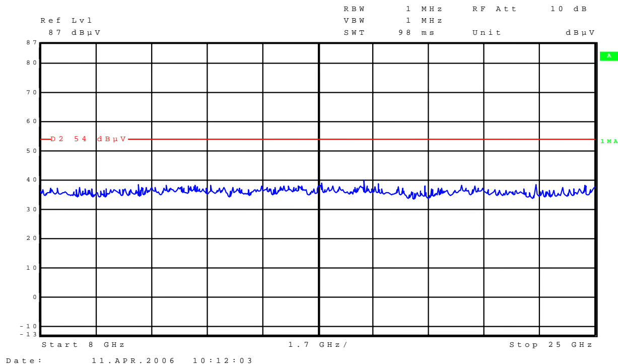
Plot 9 of 11: highest channel ( 8GHz – 25GHz)
