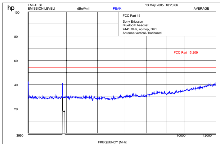
Plot : 4- 12 GHz vertical/horizontal (middle channel)
