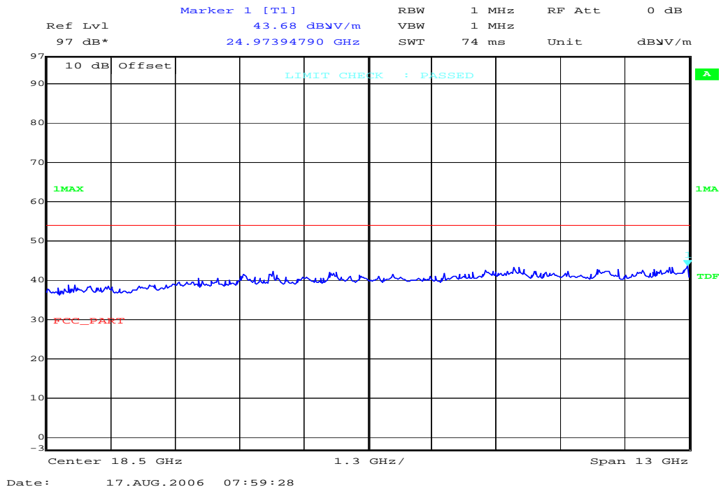
Plot : 12- 25 GHz vertical/horizontal (middle channel)
