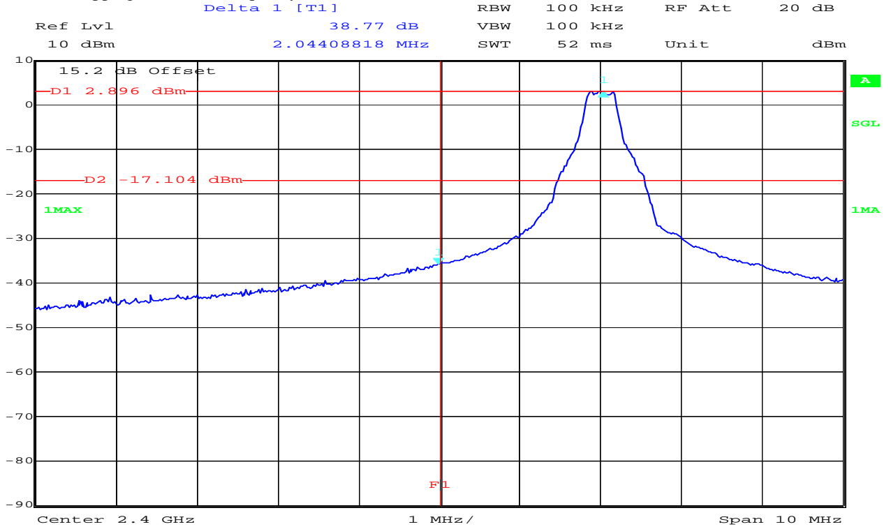
Plot 1 of 4 (hopping off, lowest frequency):
