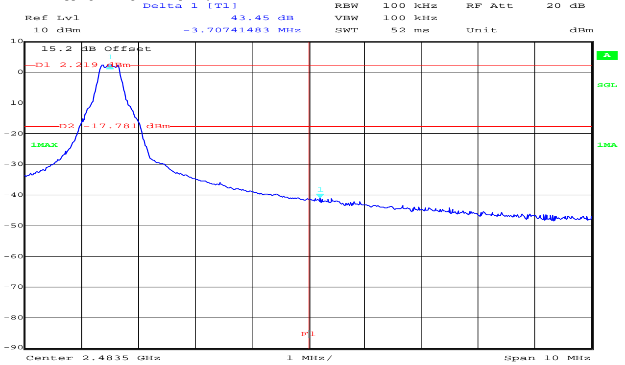
Plot 3 of 4 (hopping off, highest frequency):
