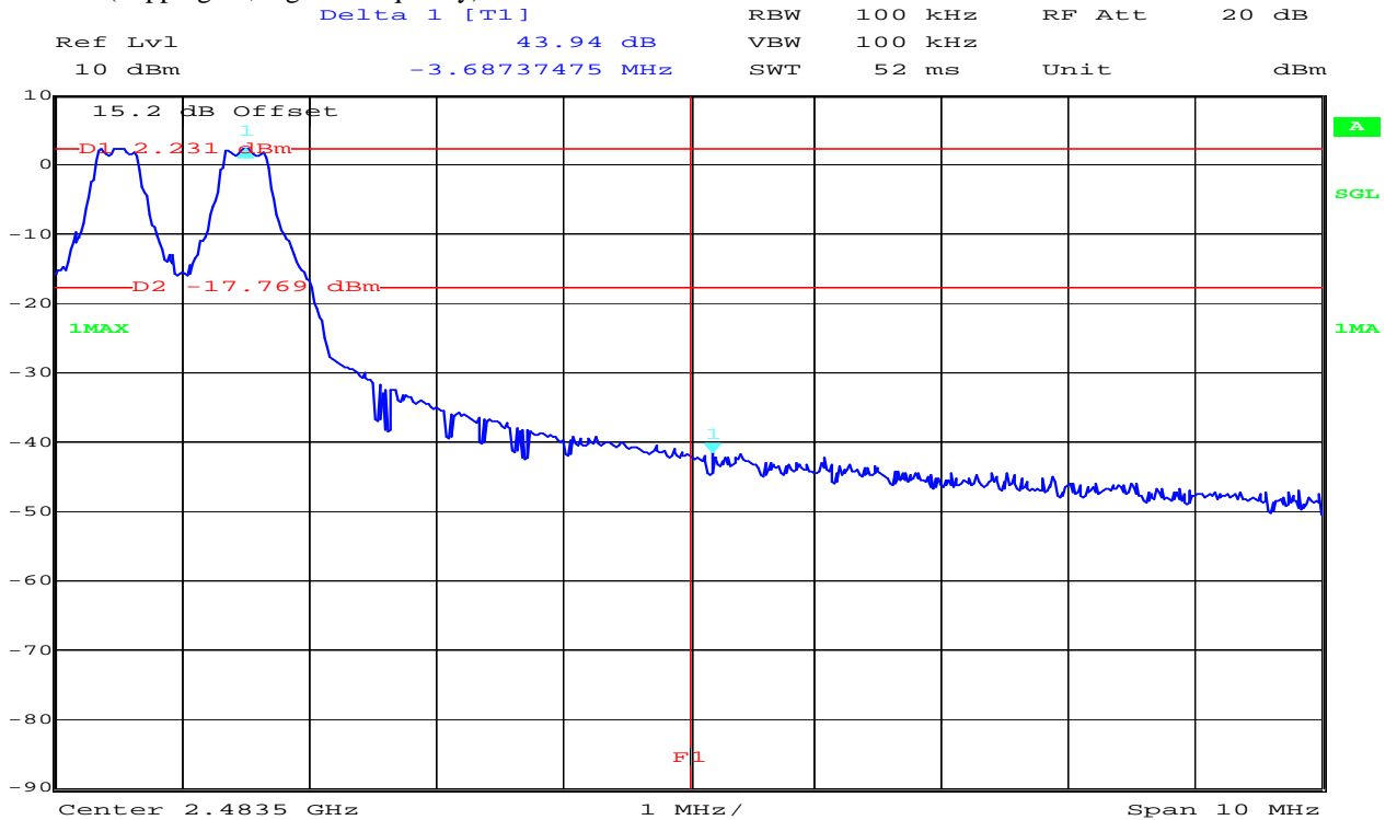
Plot 4 of 4 (hopping on, highest frequency):
