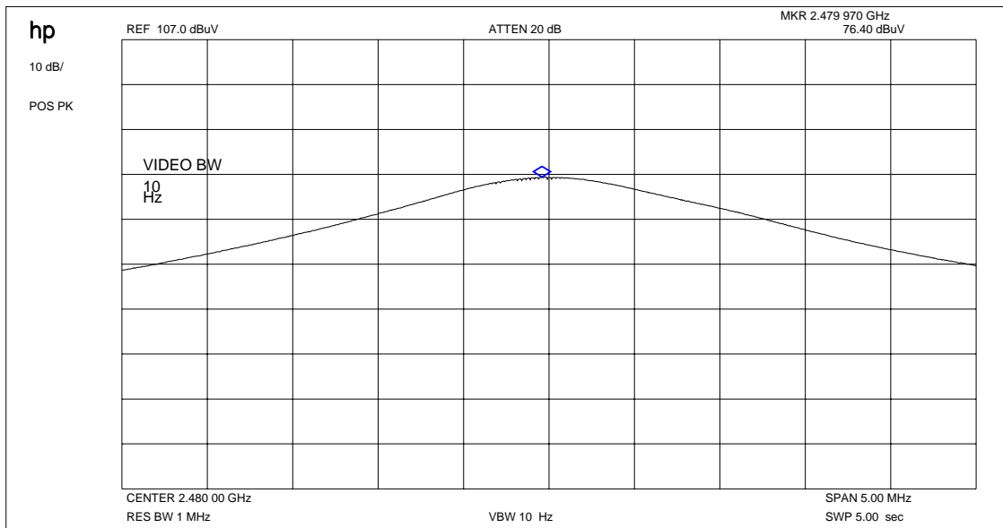
Plot 1 : Max field strength in 3m distance (single frequency)
