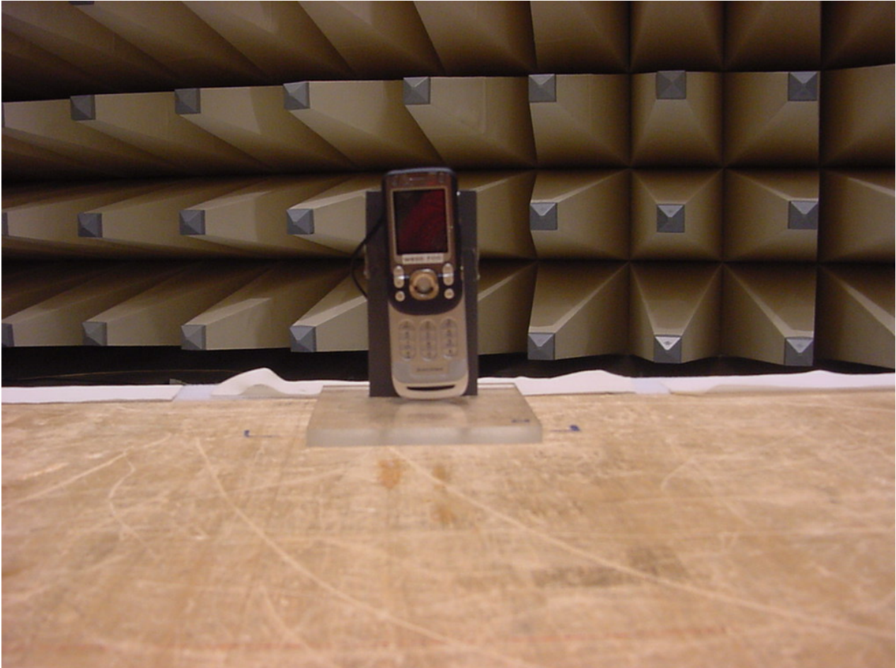
Photo 3 (Radiated Emissions):
