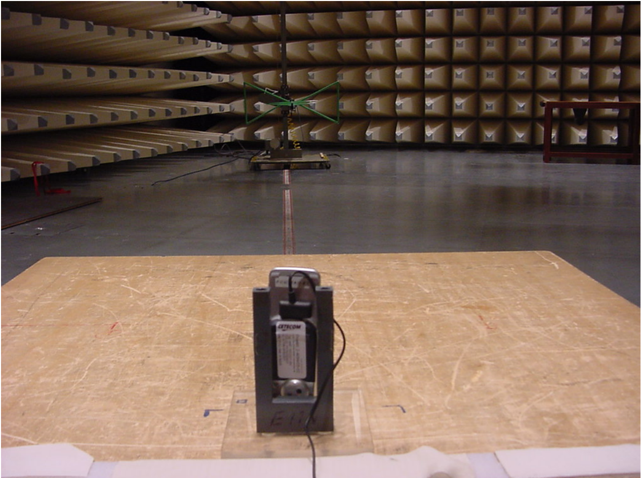
Photo 4 (Radiated Emissions):
