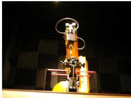
Figure 3-1 HAC RF Emissions Measurement System
