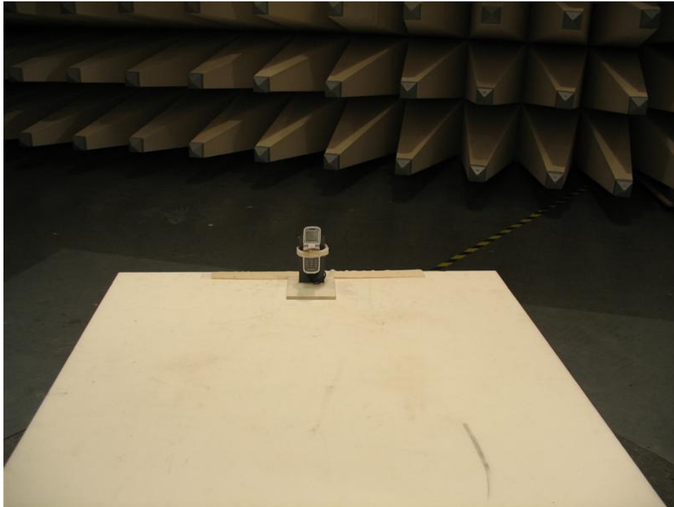
Photo 1: Radiated Emissions
