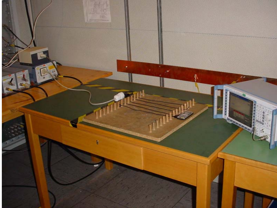
Photo 3: Conducted Emissions
