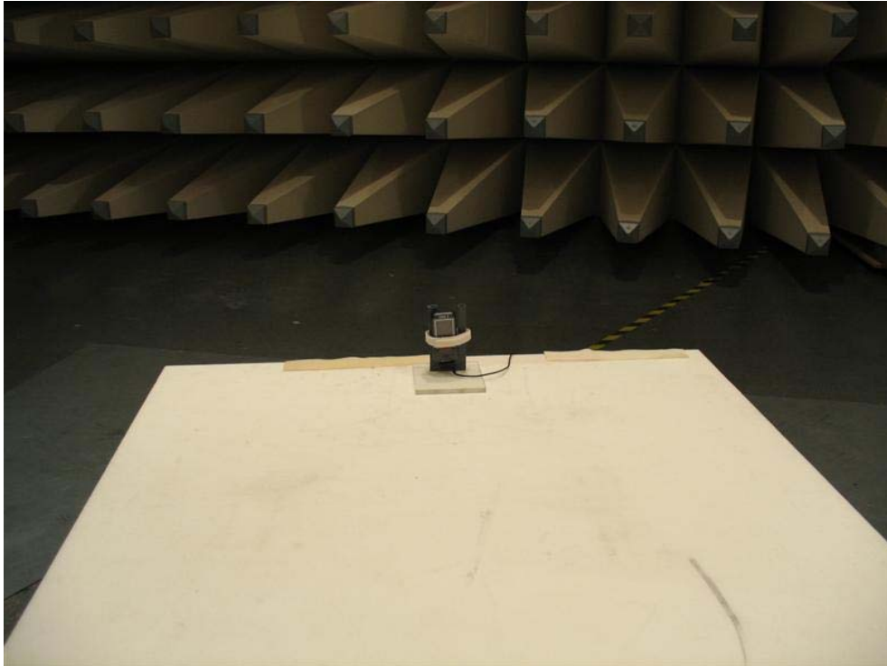
Photo 1 (Radiated Emissions):
