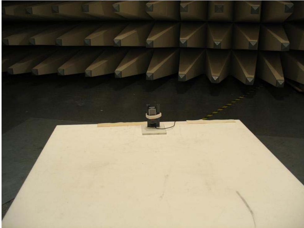
Photo 1 (Radiated Emissions):
