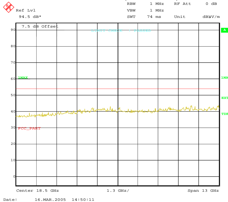
Plot : 12- 25 GHz vertical/horizontal (middle channel)
