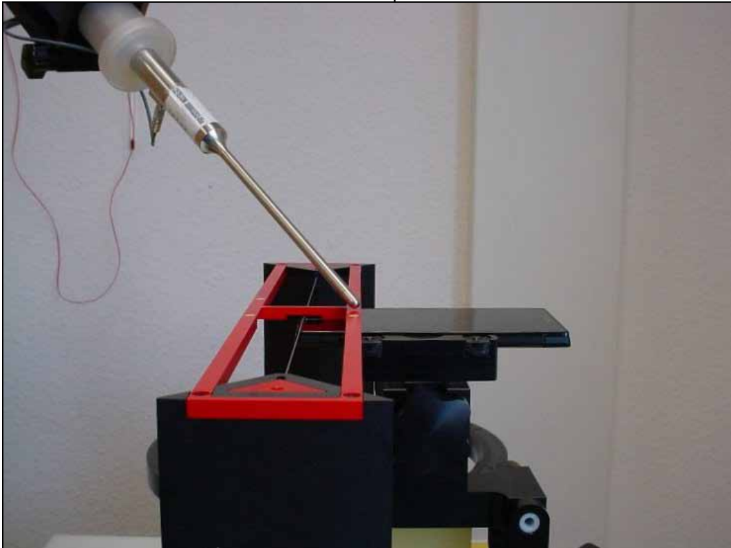
Photo 6: Test position
