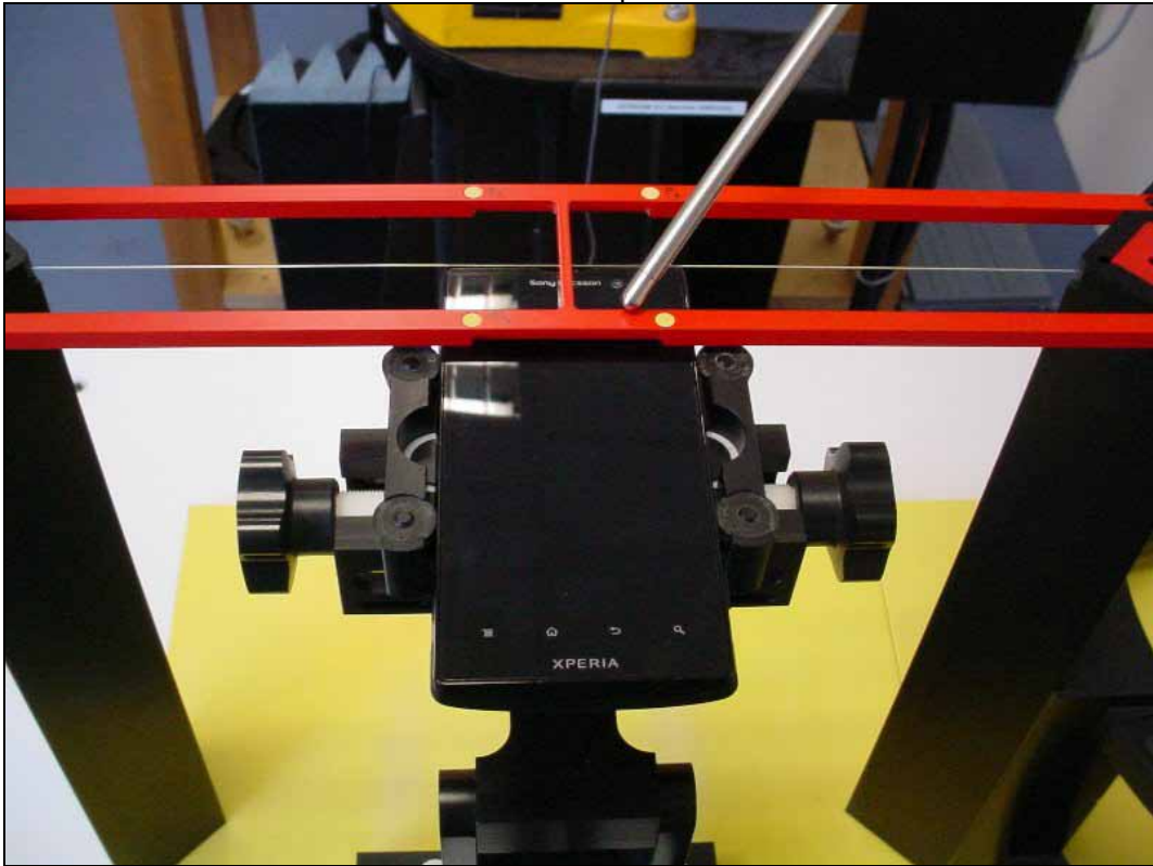
Photo 7: Test position
