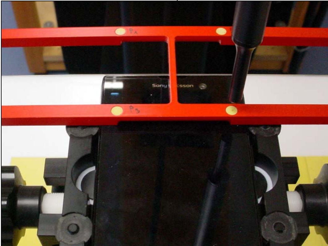
Photo 7: Test position
