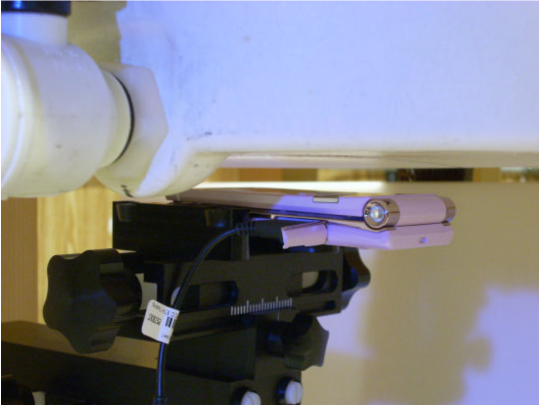
Figure 9: Body SAR, Front Side with 15mm Space
