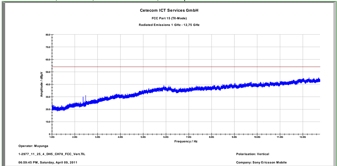
Plot 12: TX mode, channel 78, 1 GHz to 12.75 GHz, vertical polarization
