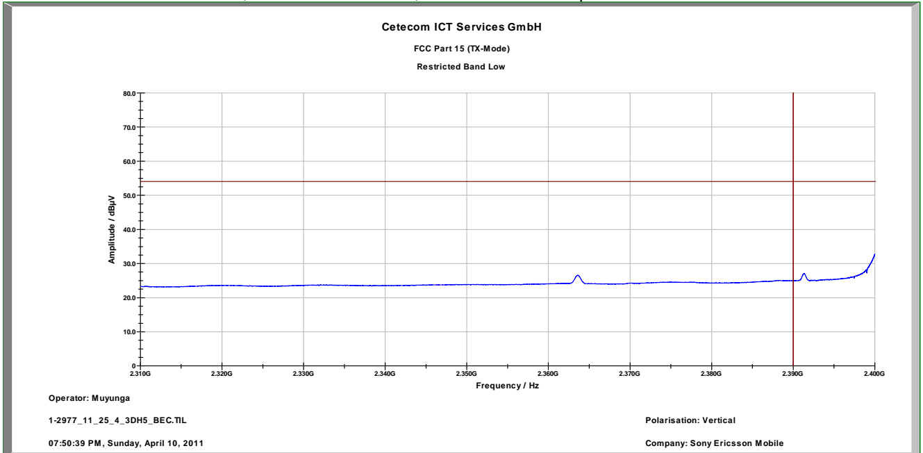
Plot 9: Lower restricted band, 8 DPSK modulation, vertical/horizontal polarization
