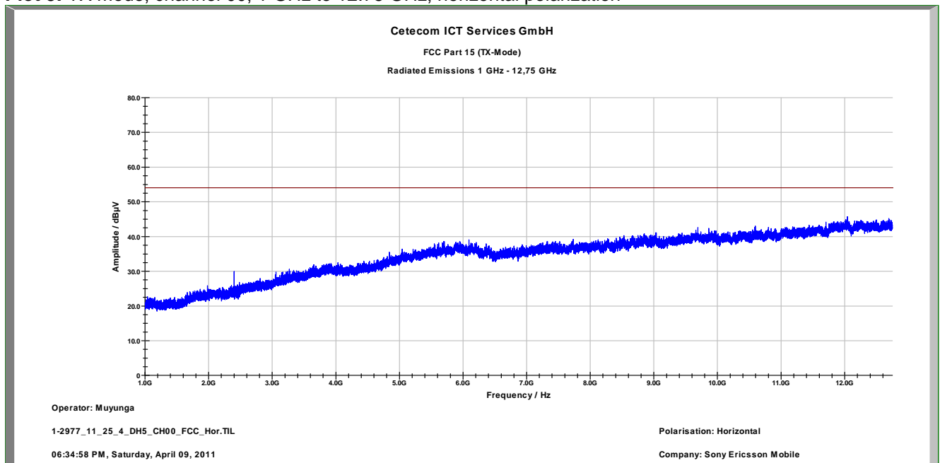
Plot 3: TX mode, channel 00, 1 GHz to 12.75 GHz, horizontal polarization
