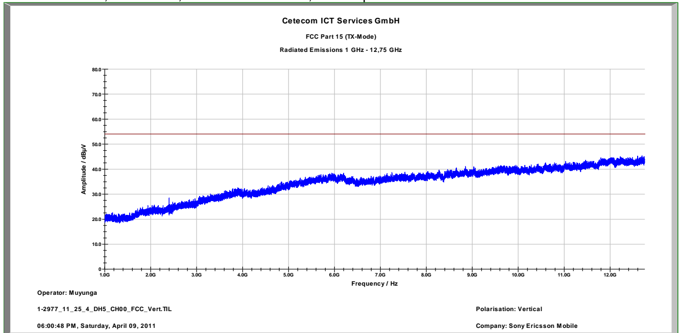
Plot 2: TX mode, channel 00, 1 GHz to 12.75 GHz, vertical polarization
