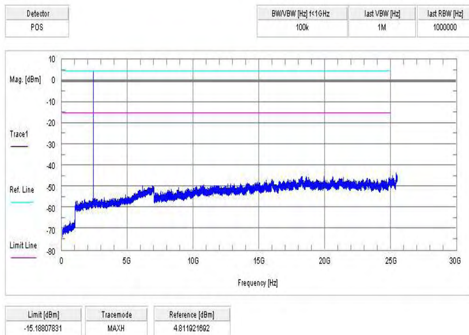
Plot 7: Channel 00 / 8DPSK
