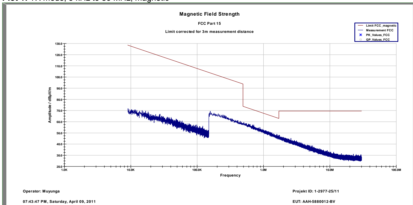
Plot 1: TX mode, 9 kHz to 30 MHz, magnetic
