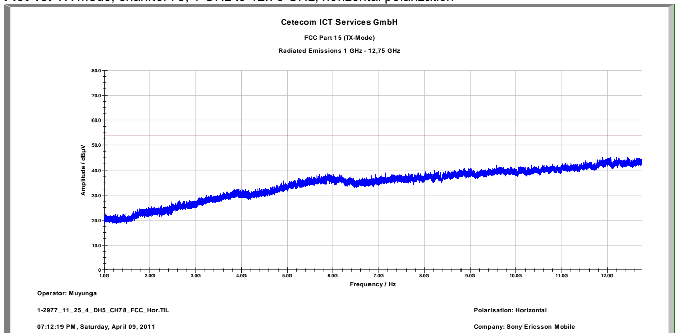
Plot 13: TX mode, channel 78, 1 GHz to 12.75 GHz, horizontal polarization
