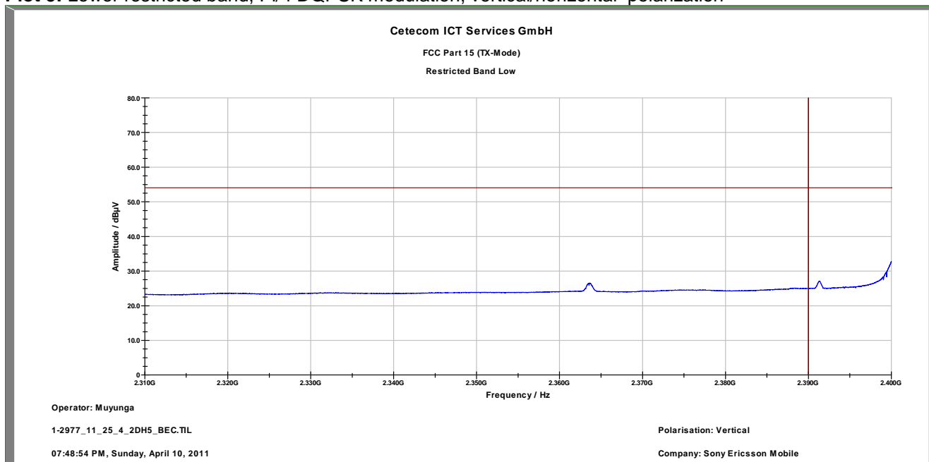
Plot 5: Lower restricted band, Pi/4 DQPSK modulation, vertical/horizontal polarization
