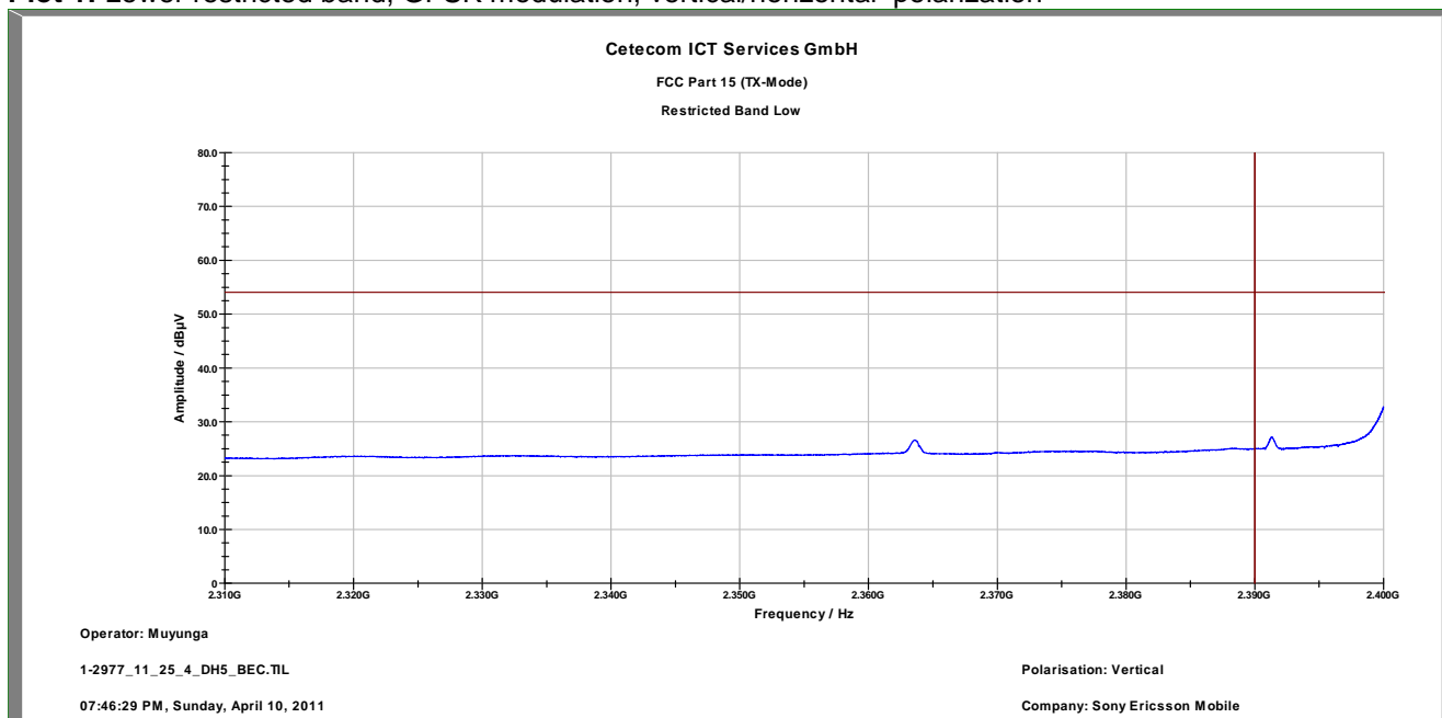
Plot 1: Lower restricted band, GFSK modulation, vertical/horizontal polarization
