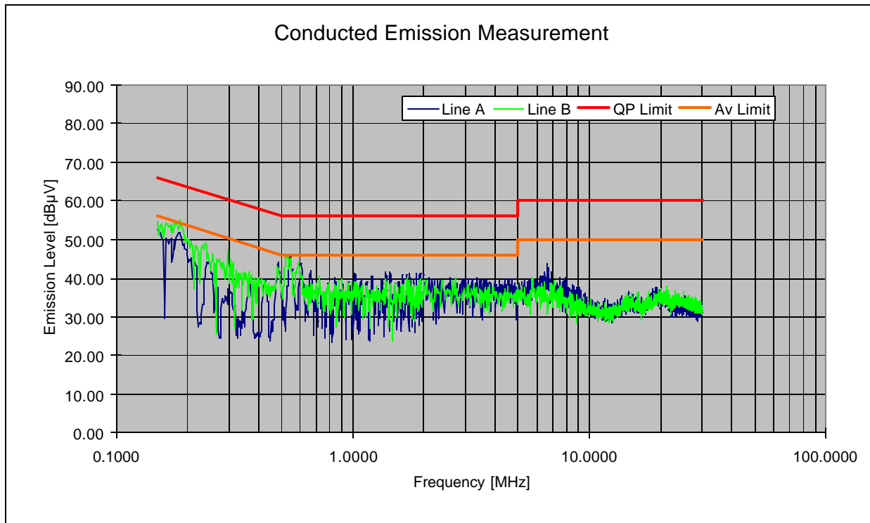
Plot 7-1. Line-Conducted Test Plot
