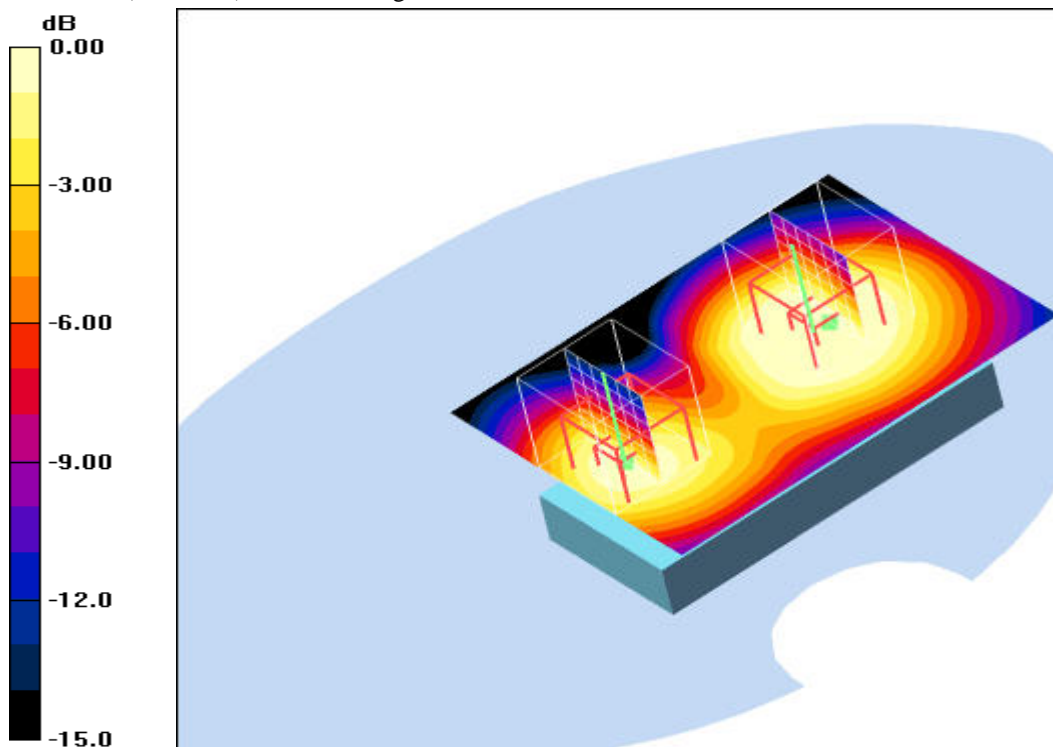
0 dB = 0.159mW/g
