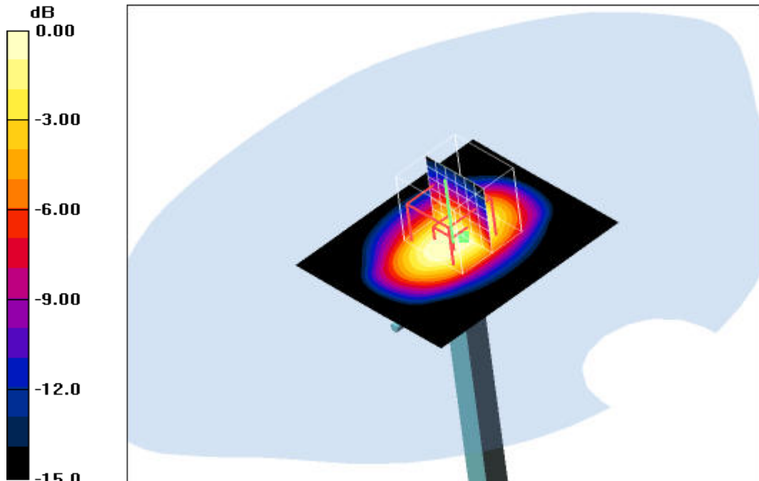
0 dB = 42.2mW/g
