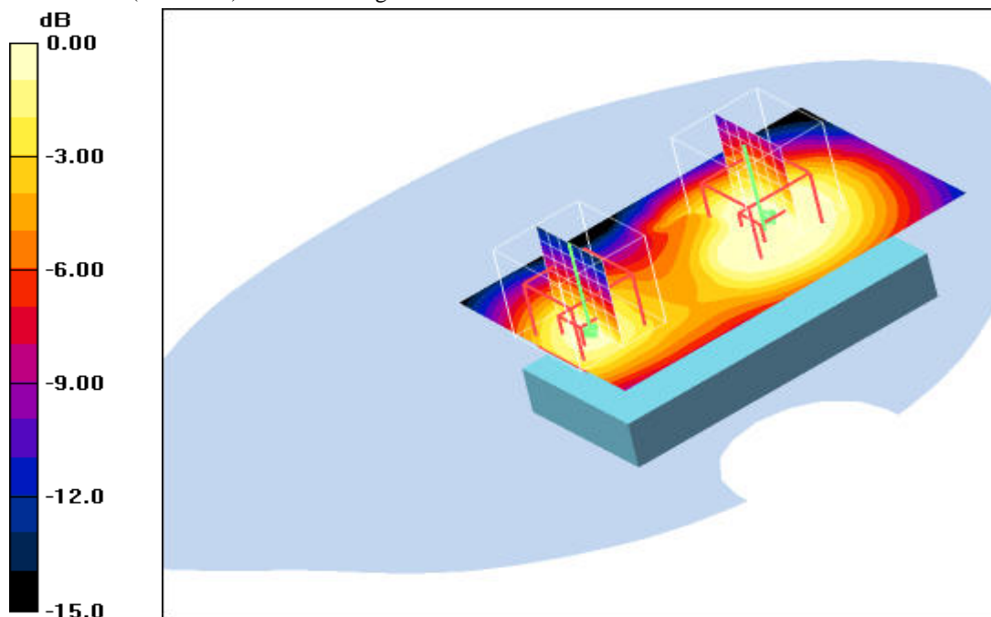
0 dB = 0.104mW/g
