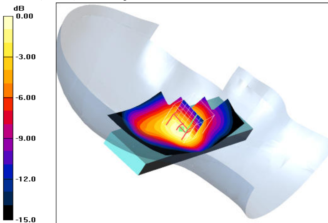
0 dB = 0.625mW/g
