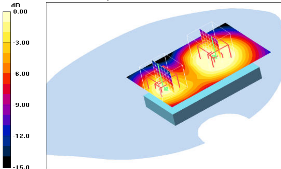
0 dB = 0.128mW/g
