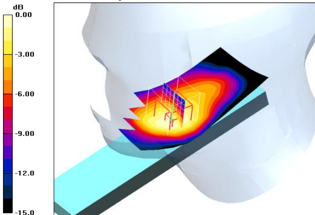
0 dB = 0.572mW/g
