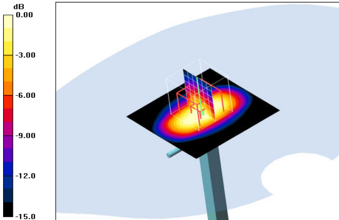
0 dB = 46.8mW/g
