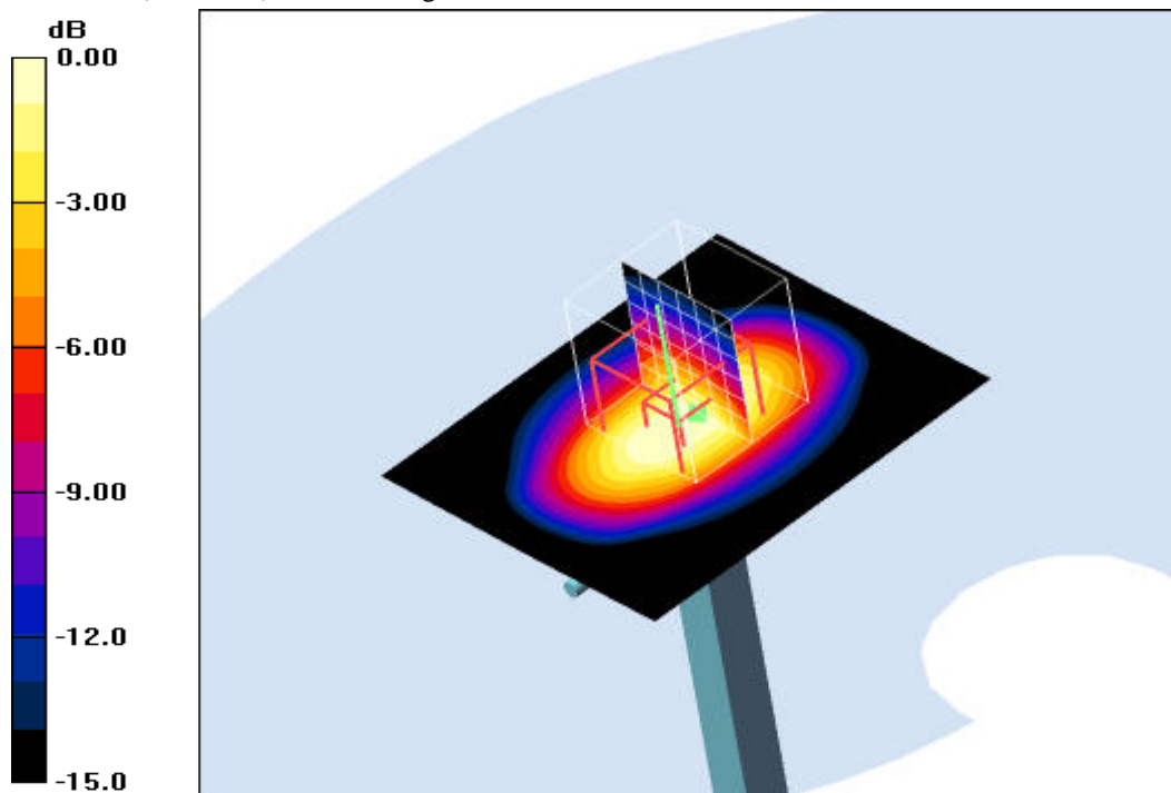
0 dB = 43.5mW/g
