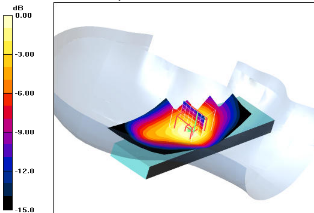
0 dB = 0.609mW/g
