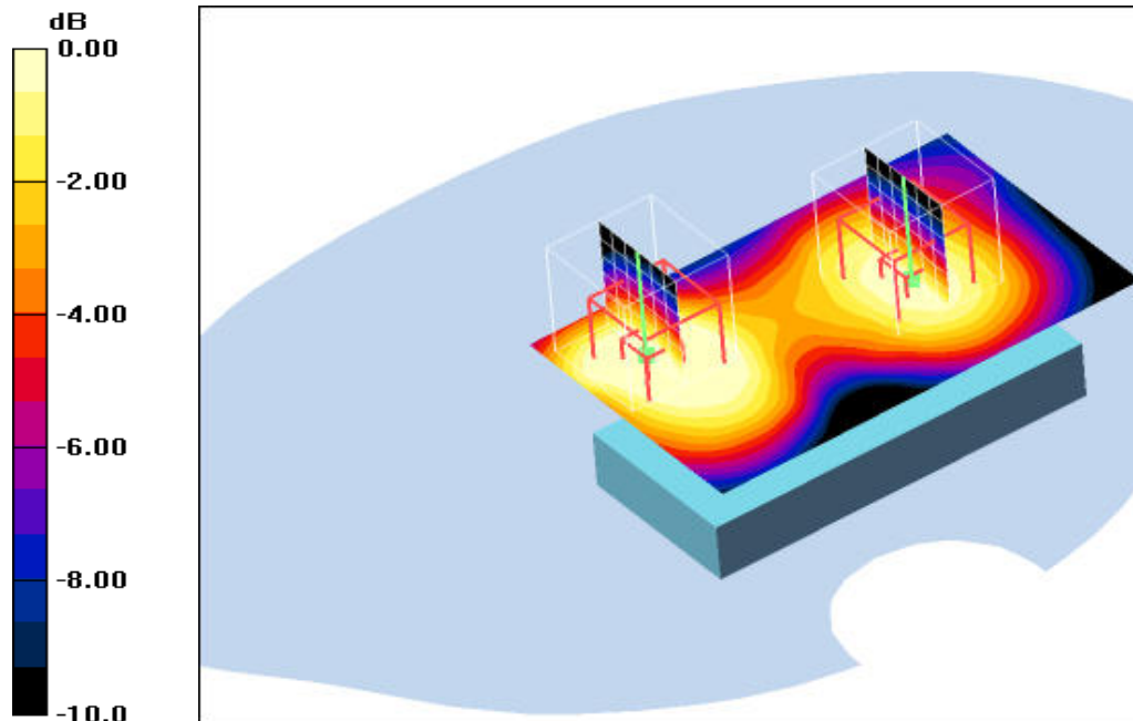
0 dB = 0.064mW/g
