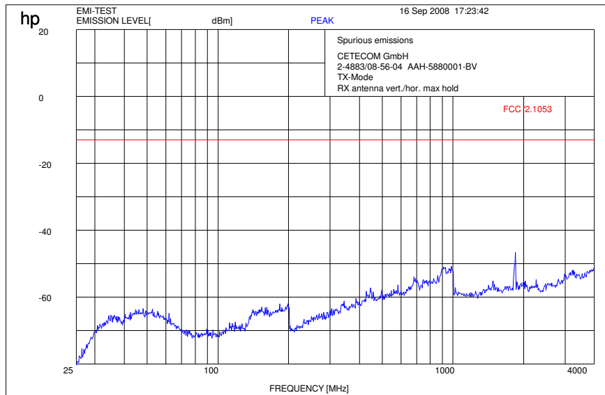
Plot 2: Traffic mode (30 MHz - 4 GHz)
