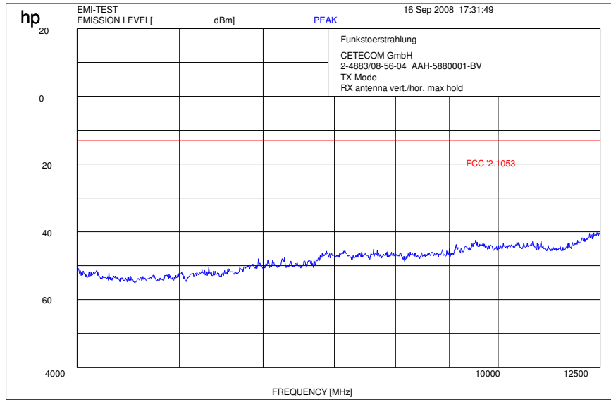
Plot 3: Traffic mode (4 GHz – 12.5 GHz)
