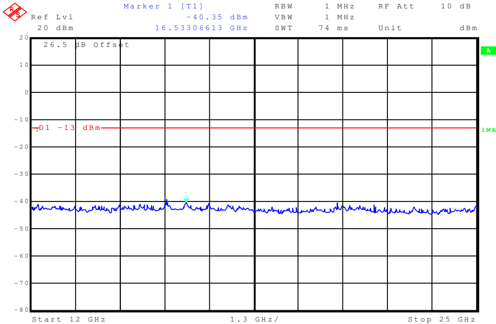
Plot 4: Traffic mode (12 GHz - 25 GHz)
