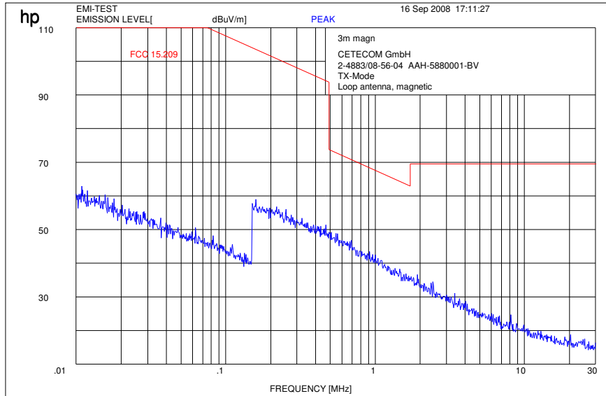
Plot 1: Traffic mode up to 30 MHz
