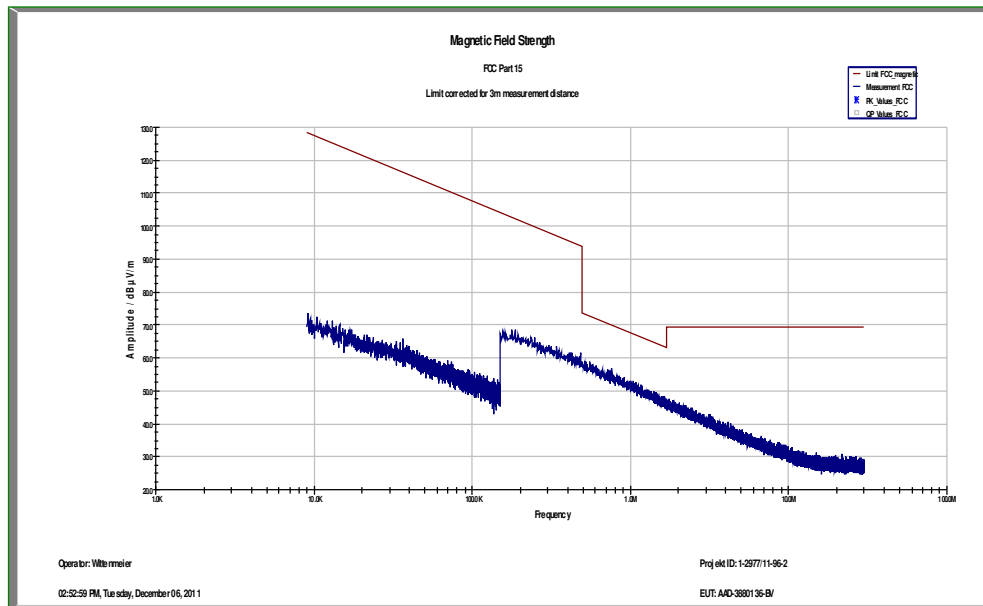
Plot 1: Receiver mode up to 30 MHz
