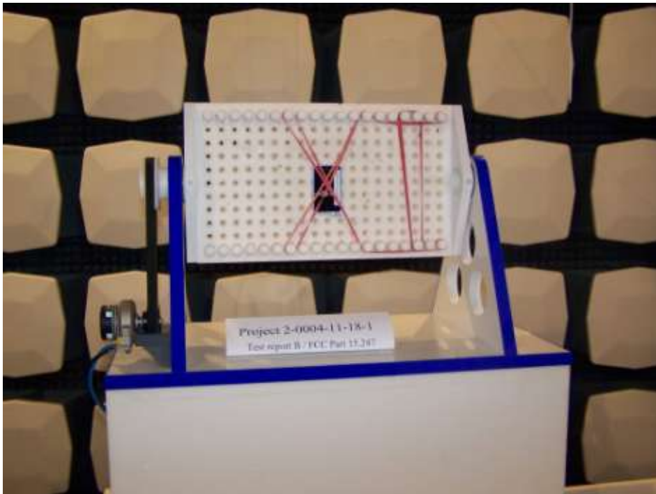
Photograph 2: Radiated test set-up: radiated RF-measurements
