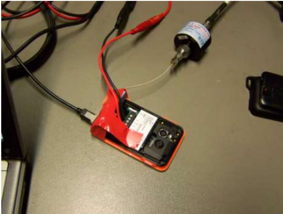
Photograph 1: Conducted test set-up: conducted RF-measurements
