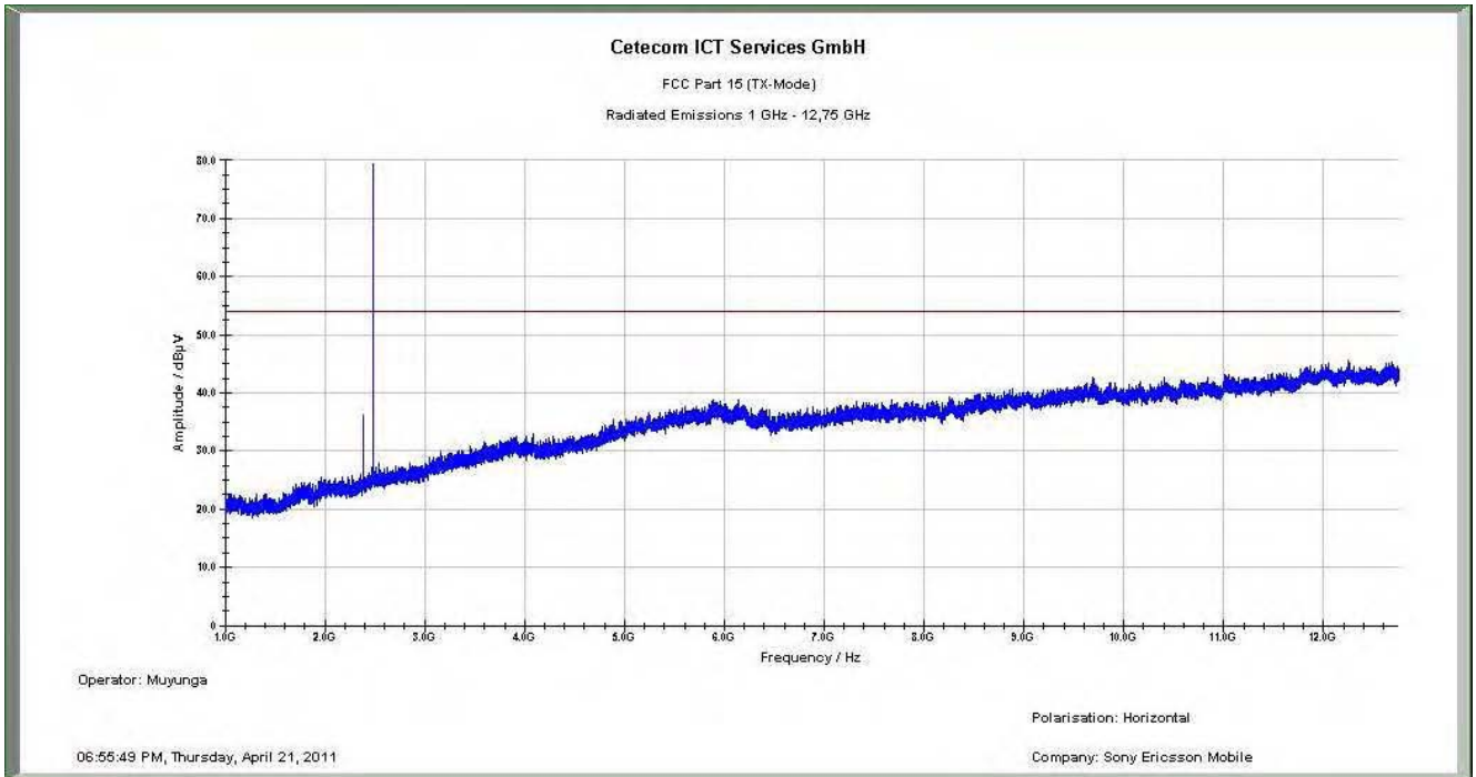
Carrier not suppressed with a 2.4 GHz-band rejection filter.
