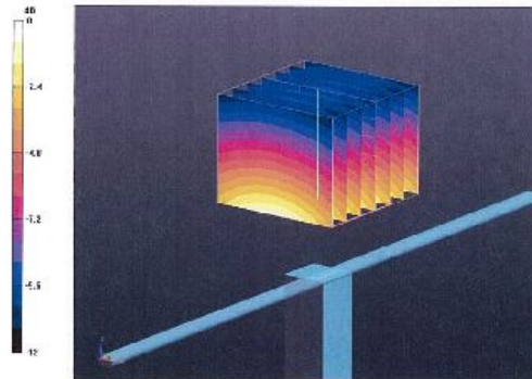
0 dB = 3.3 mW/g
