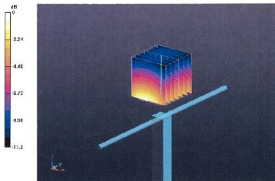
0 dB = 3.34mW/g
